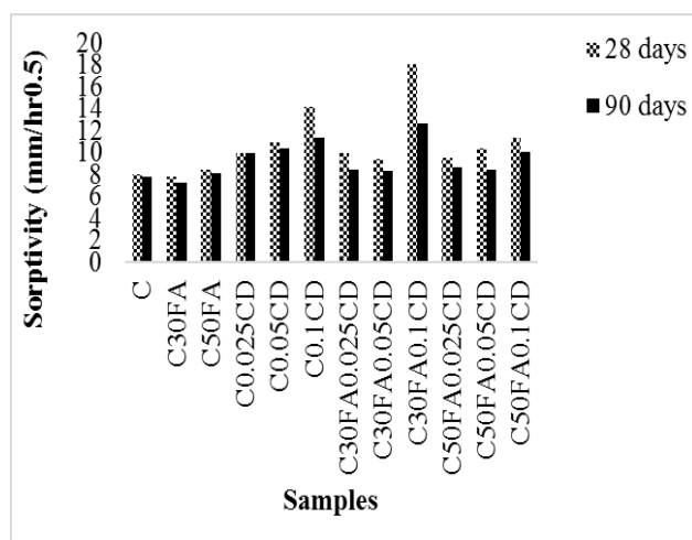
Fig. 5. Sorptivity of 0.4-W/B samples
