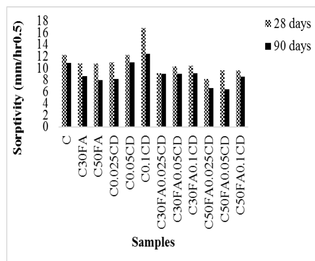
Fig. 4. Sorptivity of 0.5-W/B samples
