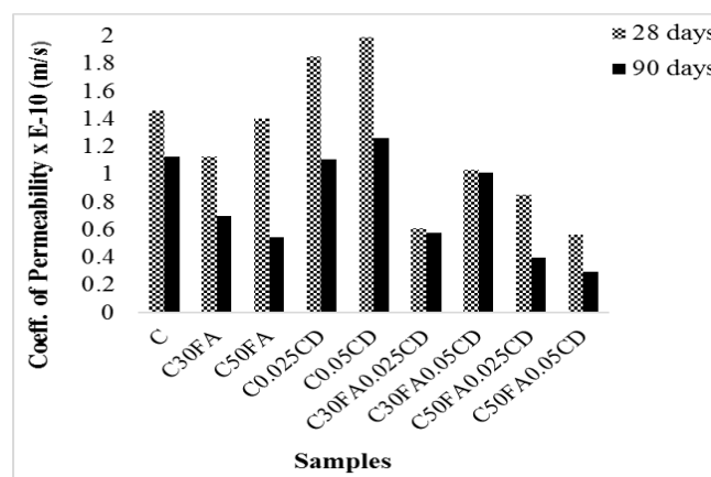
Fig. 2. Coefficient of permeability of 0.5-W/B samples
