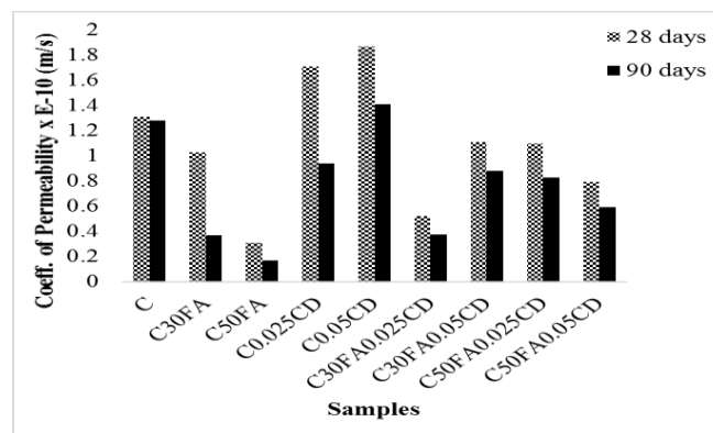
Fig. 3. Coefficient of permeability of 0.4-W/B samples
