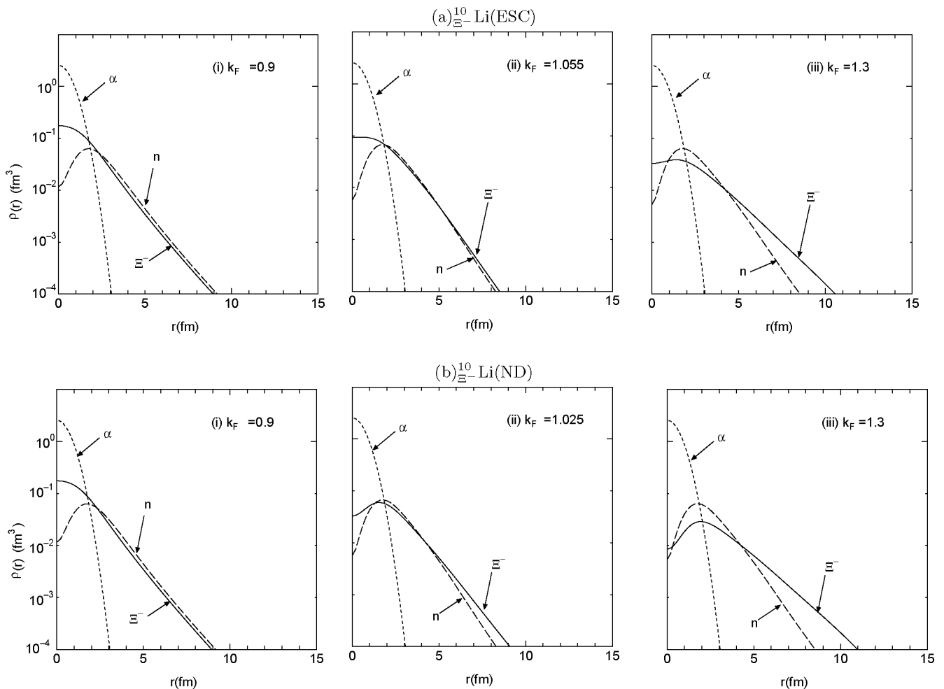
FIG. 7: (a) Calculated density distribution of \alpha , \Xi^- , and a valence neutron for three k_F values using ESC. (b) Calculated density distribution of \alpha , \Xi^- , and a valence neutron for three k_F values using ND. The wavefunctions of \alpha\Xi^- without the imaginary part of the \alpha\Xi^- interaction are used.
