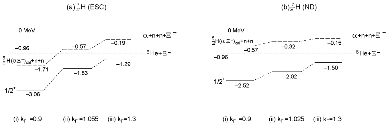
FIG. 4: (a) Calculated energy levels of {}_{\Xi}^7\text{H} for three k_F values using ESC. (b) Calculated energy levels of {}_{\Xi}^7\text{H} for for three k_F values using ND. The energies are shown when the imaginary part of the \alpha\Xi^- interaction is switched off. The energies are measured from the \alpha + n + n + \Xi^- breakup threshold. The dashed lines are threshold.
