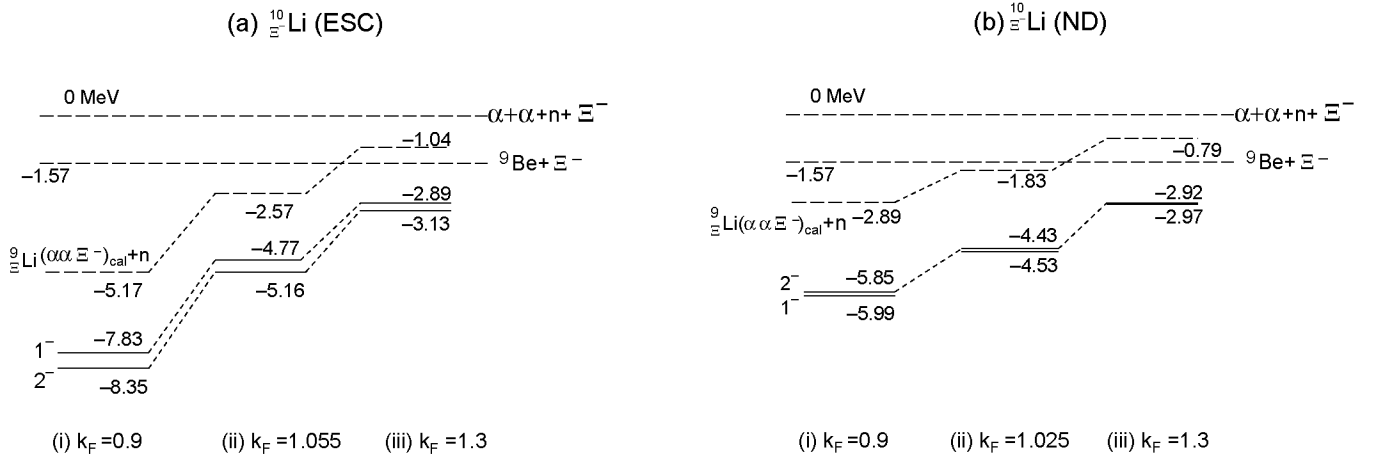
FIG. 6: (a) Calculated energy levels of ^{10}_{\Xi}\text{Li} for three k_F values using ESC. (b) Calculated energy levels of ^{10}_{\Xi}\text{Li} for three k_F values using ND. The energies are shown when the imaginary part of the \alpha\Xi^- interaction is switched off. The energies are measured from the \alpha + \alpha + n + \Xi^- threshold. The dashed lines indicate thresholds.
