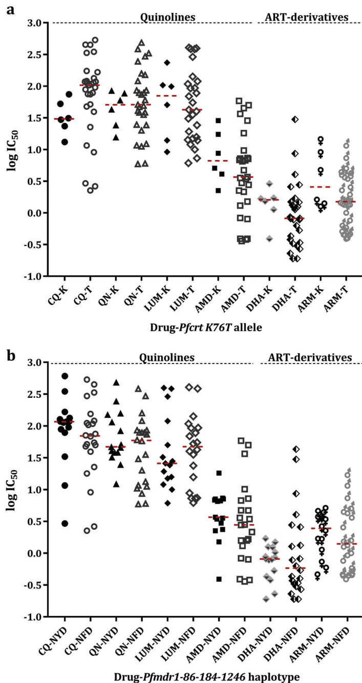
FIG 5 In vitro sensitivity (IC 50 ) of Plasmodium falciparum isolates collected in the year 2015 for mutant or wild-type alleles at pfprt K76T codon (a) and pfmdr1 -86-184-1246 haplotypes of isolates assayed against quinolines (CQ, QN, LUM, and AMD) and artemisinin derivatives (DHA and ARM) (b). Each point in a group represents the logIC 50 for an isolate with the specific allele or haplotype and drug labeled on the x axes. Broken red lines show the median logIC 50 values for each haplotype group per drug.
