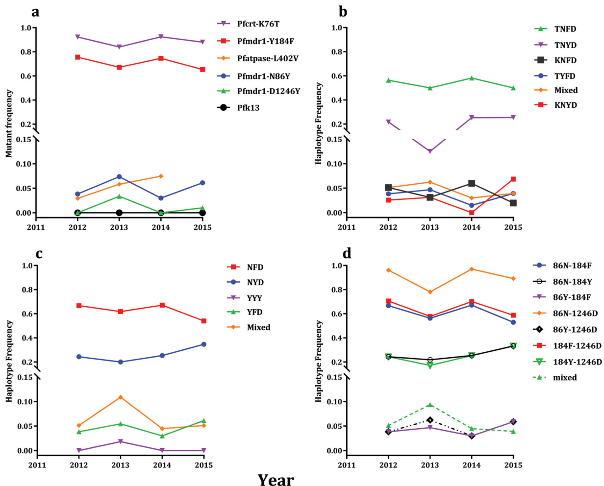
FIG 4 Temporal trends in the frequencies of Plasmodium falciparum drug resistance alleles at chloroquine resistance transporter ( pfprt ), multidrug resistance protein 1 ( pfmdr1 ), and calcium-transporting ATPase ( pfatpase6 ) (a), pfprt - pfmdr1 haplotypes (b), pfmdr1 codons 86-184-1246 haplotypes (c), and biallelic haplotypes at pfmdr1 codons 86, 184, and 1246 (d). Isolates were collected across four transmission seasons (years 2012 to 2015) from Brikama, The Gambia. Each point represents the frequency (y axes) plotted against the year (x axes) isolates were collected. Each line shows the trend for frequencies of alleles or haplotypes in the figure legends.
