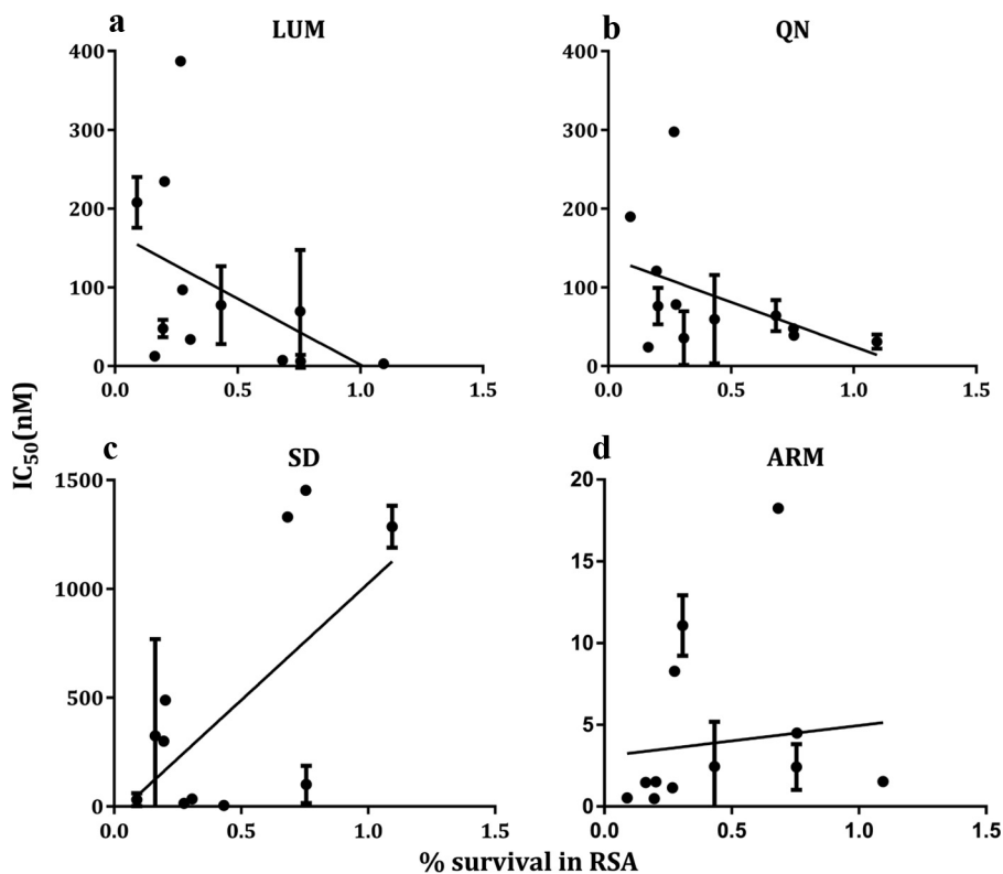
FIG 3 Correlation between drug IC_{50} s (y axes) for LUM (a), QN (b), SD (c), and ARM (d) and the percentage of rings surviving after dihydroartemisinin exposure. Each point corresponds to the IC_{50} plotted against the percentage of infected cells with parasite growth for an isolate, with the confidence interval of the IC_{50} shown as bars.
