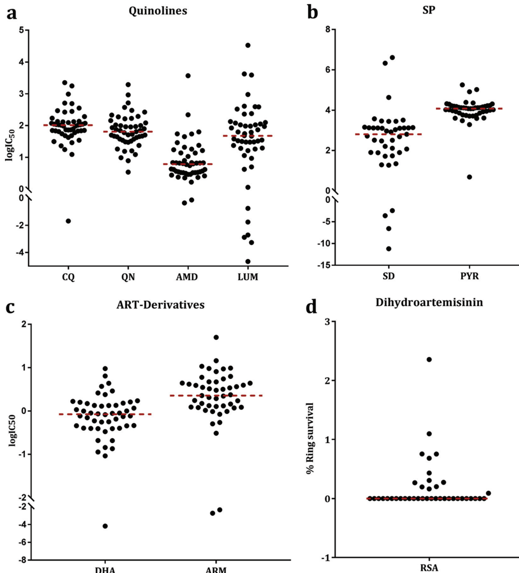
FIG 2 In vitro drug susceptibilities of Plasmodium falciparum isolates collected in the year 2015 from Brikama determined by flow cytometry (ACCURI) and IVART for standard inhibitory drug concentrations ( IC_{50} ) and RSA against dihydroartemisinin. The \log IC_{50} for each isolate is shown for quinolines (chloroquine [CQ], quinine [QN], AMD, and LUM) (a), SP drugs sulfadoxine (SD) and pyrimethamine (PYR) (b), and artemisinin derivatives DHA and ARM (c). (d) RSA. The percentage of infected cells with parasite growth after DHA treatment of ring stages for each isolate is shown. Broken red lines are the median value of the isolates for each assay.
