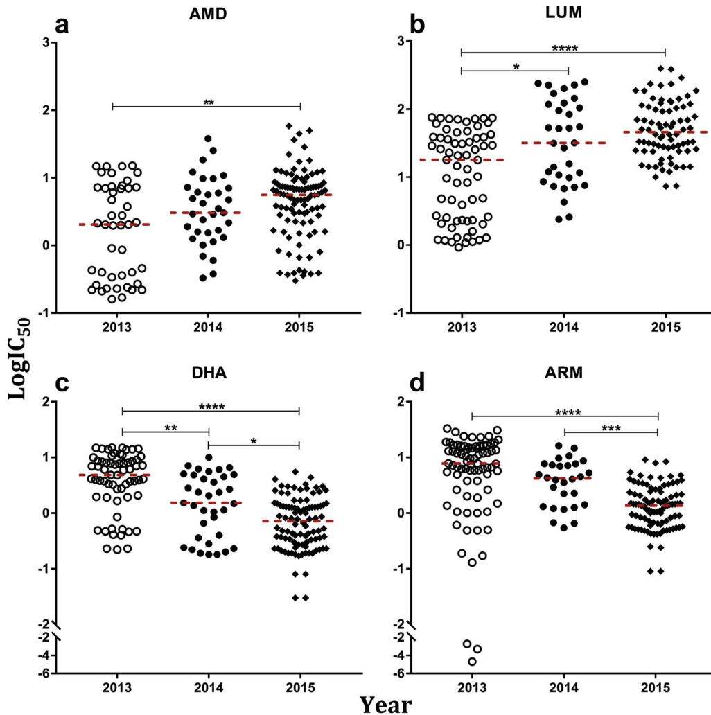
FIG 1 In vitro drug susceptibilities of Plasmodium falciparum isolates collected from Brikama (western Gambia) during the transmission seasons from years 2013 to 2015. Each plot shows the \log_{10} of the 50% inhibitory concentration ( \log IC_{50} ) of isolates for a drug grouped per year of isolate collection as labeled on the x axes. Each point is the \log IC_{50} for an isolate against amodiaquine (AMD) (a), lumefantrine (LUM) (b), dihydroartemisinin (DHA) (c), and artemether (ARM) (d). The median for each drug per year is shown as broken red lines. Lines connect pairs of years for which the distribution of IC_{50} s were significantly different at a P value of <0.05 (*). The most significant differences had P values of <0.0001 (****).
