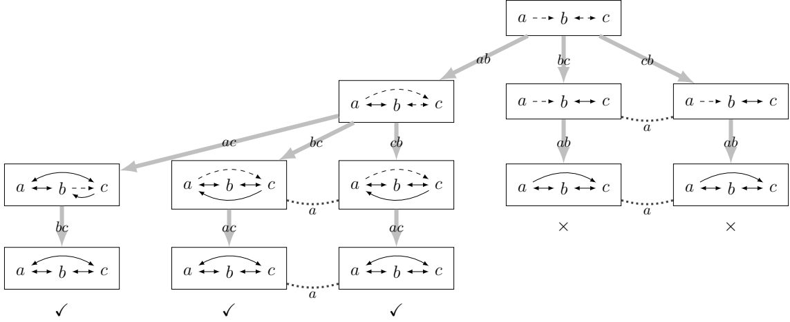
Figure 1: Example of an execution tree for LNS .
