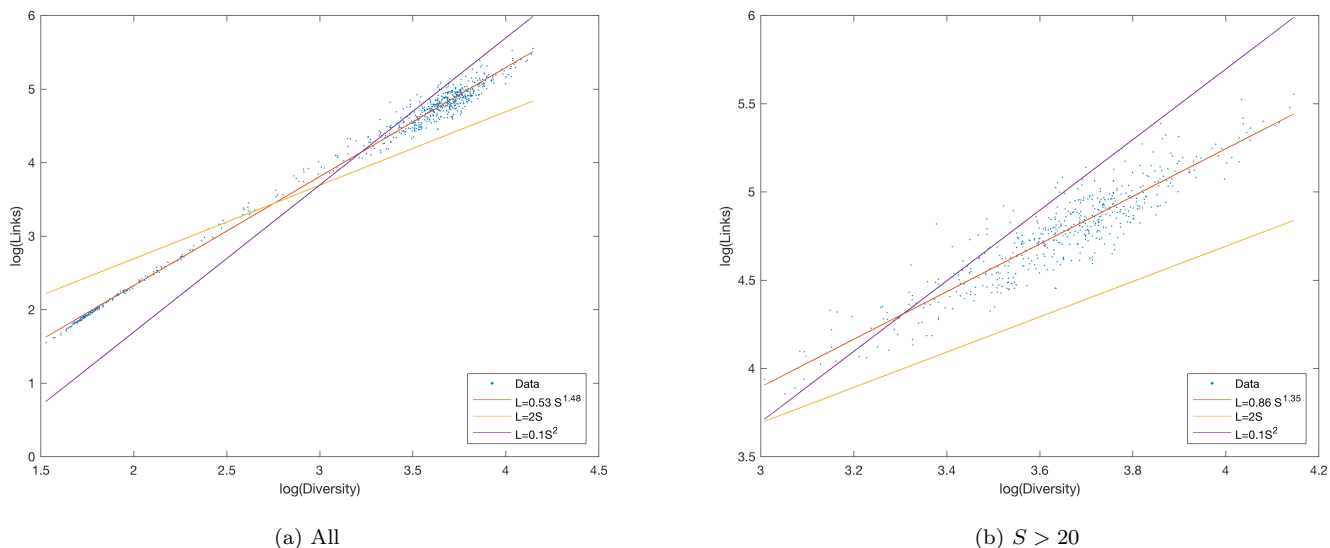
Figure 12: Link-Species Relationship for Taxonomic Webs 4
