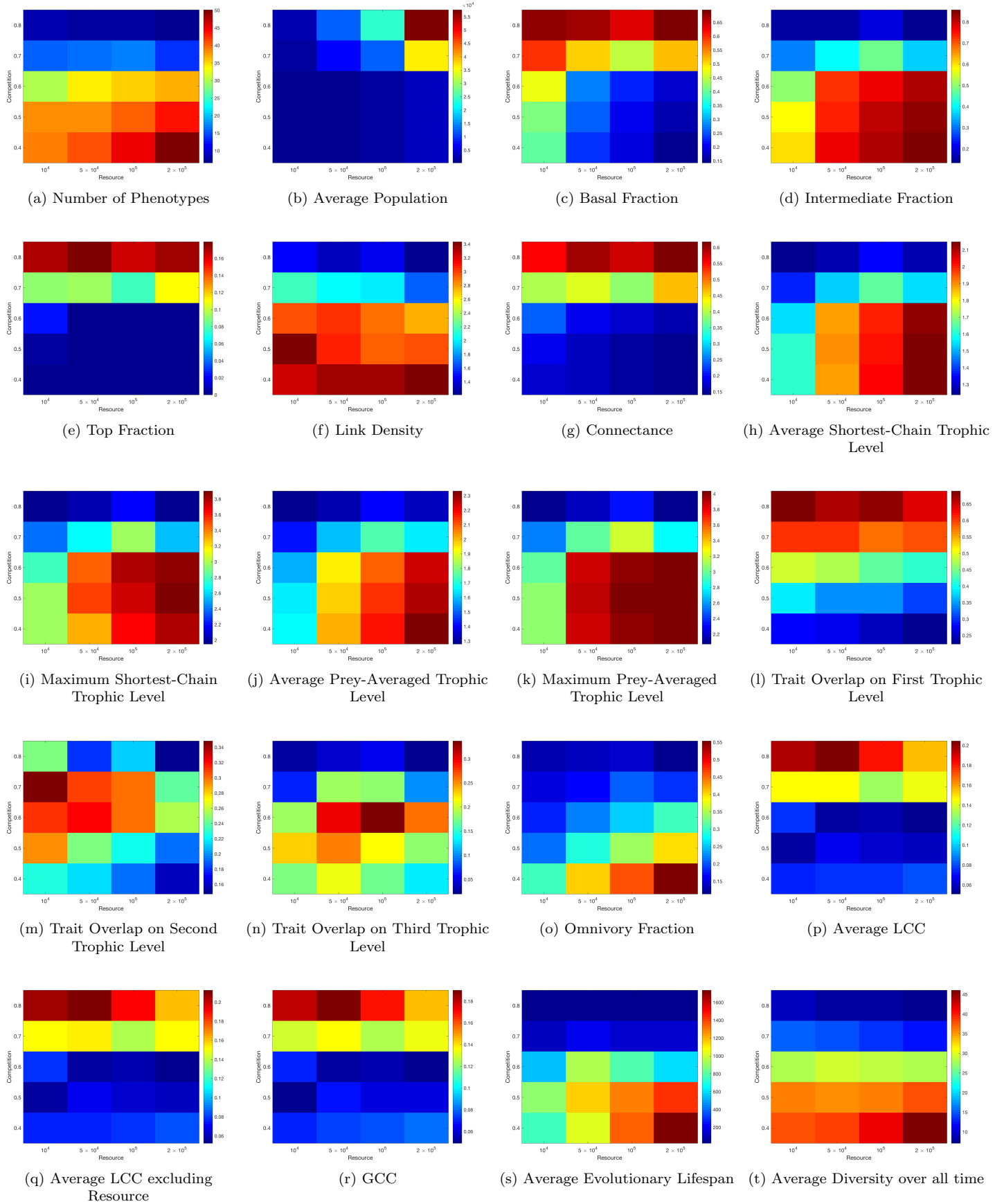
Figure 9: Averaged Data of Taxonomic Webs
