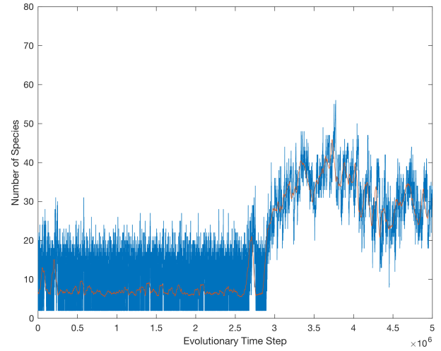
(b) c = 0.7, R = 10^{-4}
