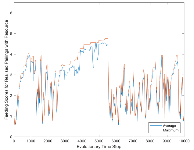
(b) Early Simulation
