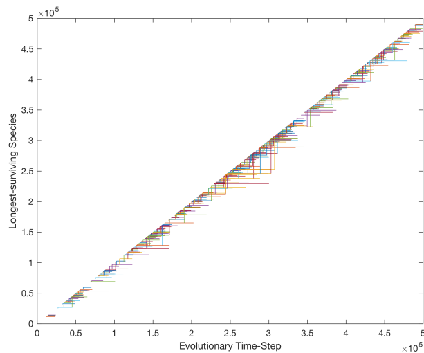
(b) 500 Longest-surviving Species
