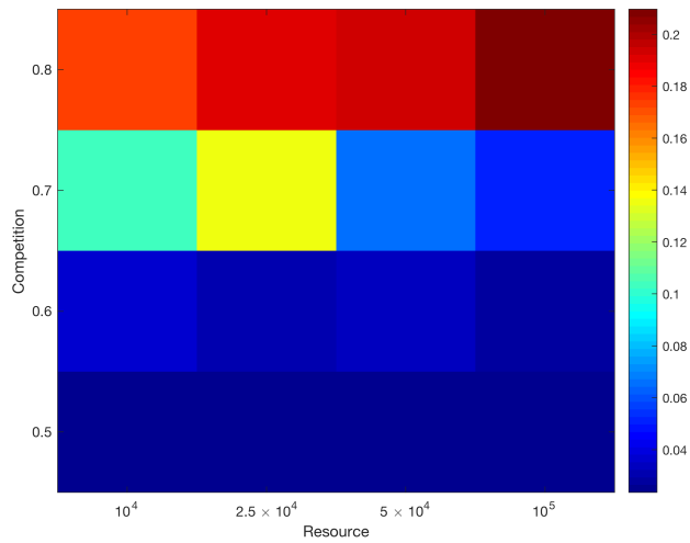
Figure 24: Average Fractional Extinction event sizes per Model Parameters
