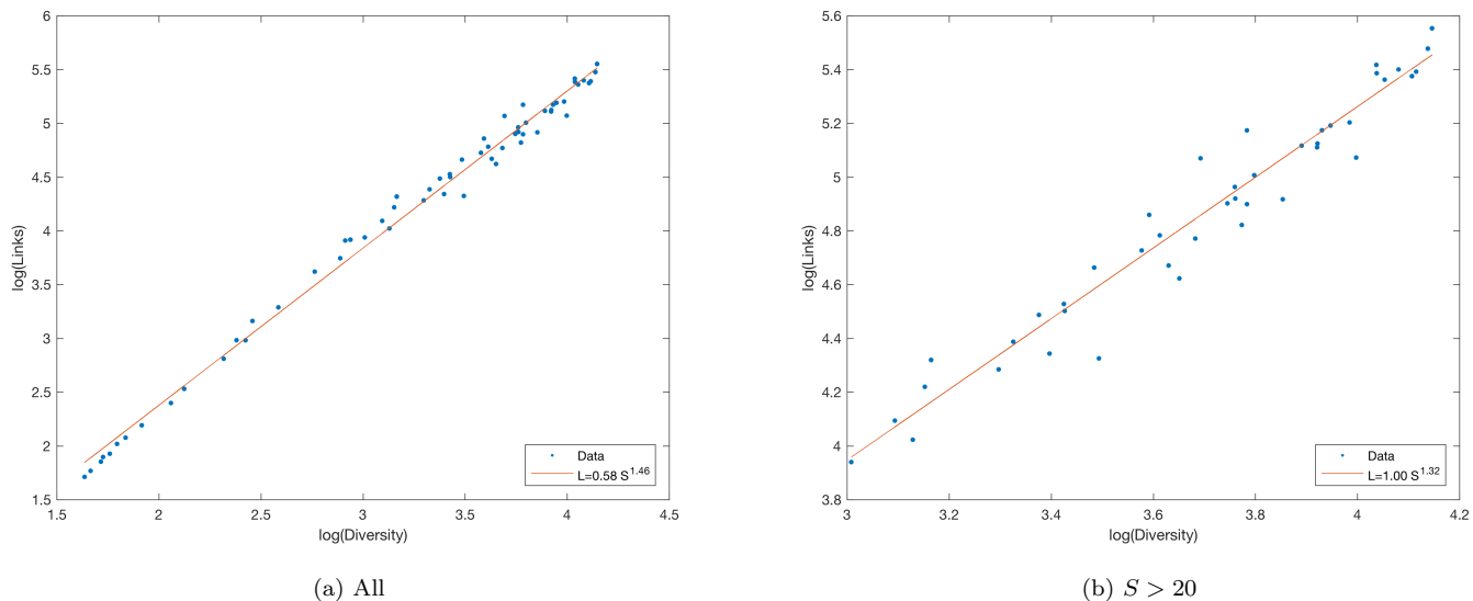
Figure 14: Taxonomic \log(\text{Links}) - \log(\text{Diversity}) Best Fit, uniformly sampled
