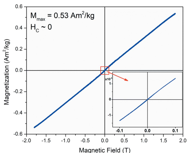
Figure 3 Magnetization–magnetic field curve of the crystallized \text{Na}_5\text{FeSi}_4\text{O}_{12} phase.
