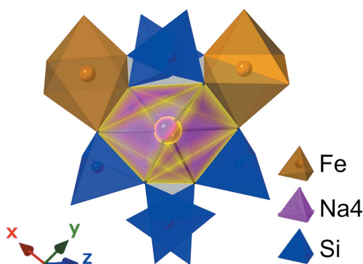
Figure 7 The tetrahedrally distorted Na4 octahedron.
