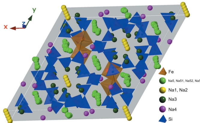
Figure 5 A mixed polyhedral and ball-and-stick representation of the unit cell of \text{Na}_5\text{FeSi}_4\text{O}_{12} . Unique Na atoms are depicted with contrasting colours.
