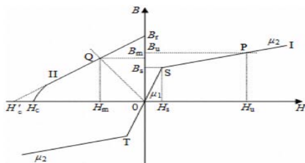
Fig. 1. Linearized B-H characteristics of active materials in PMFCL [5]
