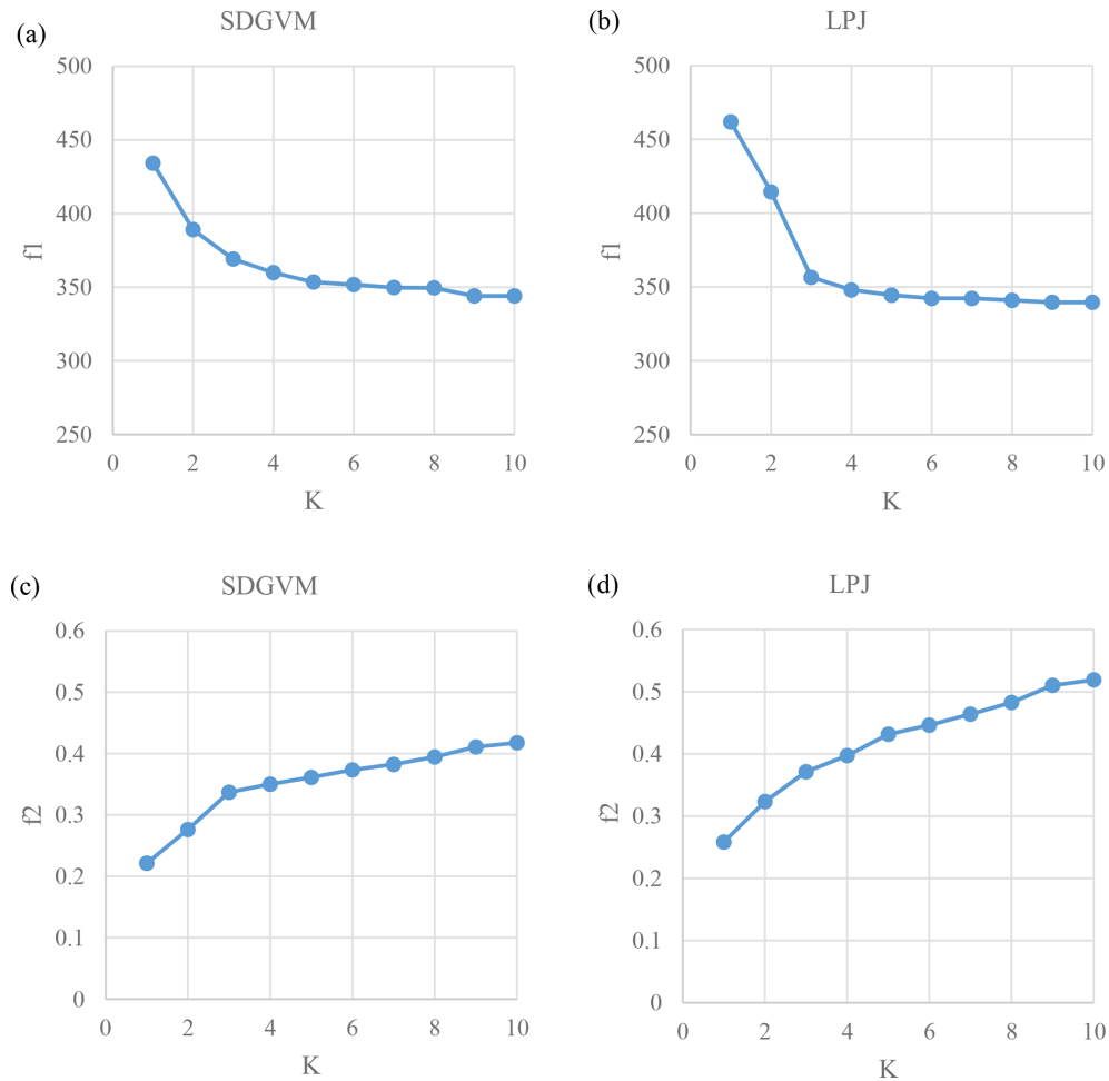
Figure 6. Variations of statistics for a match between Eocene maxKNN predicted high FW and coal locations (Boucot et al., 2013). The f_1 is the mean distance of a coal location to site with FW > 0.2 for model based on (a) SDGVM and (b) LPJ. The f_2 is the mean FW of sites within 2 pixels of a coal location for model based on (c) SDGVM and (d) LPJ data.
