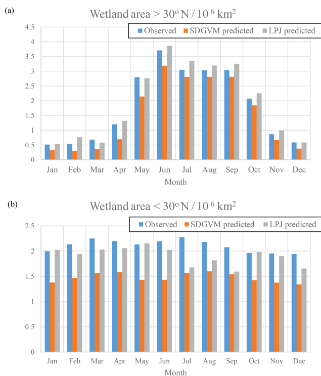
Figure 3. Monthly zonal variations in FW calculated for the mean 2000–2012 climate on a 2.5^\circ \times 3.75^\circ grid; (a) north of 30^\circ N and (b) south of 30^\circ N.
