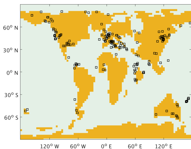
Figure 5. Locations of Eocene coal deposits plotted on our Eocene model land mask. The □ symbols indicate an Eocene coal deposit location (Boucot et al., 2013).
