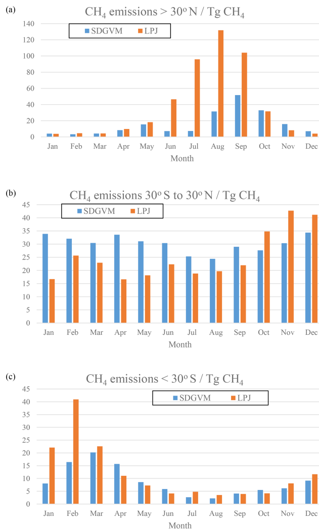
Figure 9. Monthly variations in wetland \text{CH}_4 emissions ( \text{Tg CH}_4 ) calculated from predicted FW for the Eocene climate by SDGVM and LPJ, for (a) all areas north of 30^\circ \text{N} , (b) all areas between 30^\circ \text{S} and 30^\circ \text{N} and (c) all areas south of 30^\circ \text{S} .
