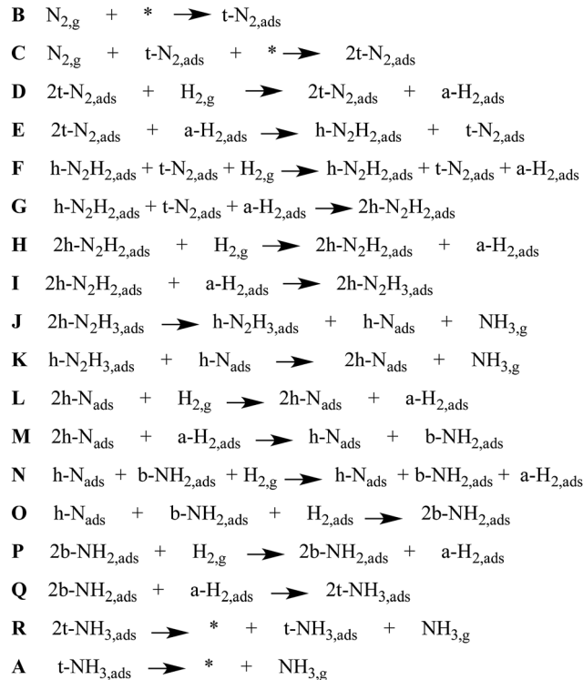
Scheme 1 Elementary reaction mechanism steps of ammonia synthesis via an Eley–Rideal mechanism on θ-Mn 6 N 5 -(111). The letters t -, b -, h - and a - are to indicate the adsorption position which is top, bridge, 3-fold hollow and adsorbate, respectively.
