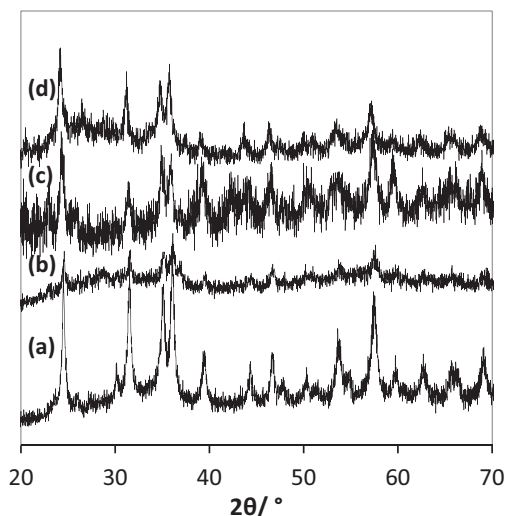
Fig. 5. XRD patterns collected after the ammonolysis step of (a) C- \text{Ta}_2\text{O}_5 , (b) \text{Ta}_{2.75}\text{Co}_{0.25}\text{N}_y , (c) \text{Ta}_{2.5}\text{Co}_{0.5}\text{N}_y , (d) \text{Ta}_2\text{CoN}_y .
