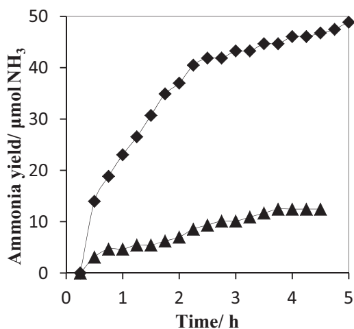
Fig. 8. Ammonia yield for \text{Ta}_3\text{N}_5 reduction with 60 \text{ ml min}^{-1} of 1:3 Ar: \text{H}_2 at T=500^\circ\text{C} : \blacktriangle A- \text{Ta}_3\text{N}_5 , \blacklozenge C- \text{Ta}_3\text{N}_5 .
