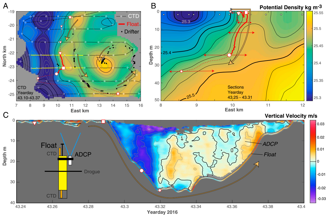
Fig. 6. Sinking of water at the front. (A) Surface density colored and contoured using same color map as in Fig. 5. Thin lines show ship survey lines; yellow lines indicate the section plotted in B; circles show stations. Mapping uses objective analysis with a 1.2-km Gaussian correlation function. Black dots show drifter positions with 5,200-s tails, the duration of the survey. (B) Section of potential density using all data along yellow tracks ( SI Float Navigation ). Small white dots show profile locations. Data are smoothed with 2 m vertical and 500 m horizontal scales. (C) Sketch of the Lagrangian float and vertical velocity (colors) computed from its data. Float was deployed at the location of the top star in A and recovered at the bottom star. Estimated trajectory ( SI Float Navigation ) is shown by the red lines in A and B and marked by white symbols common to all panels. Solid lines are more certain than dashed ones. Horizontal arrows in B indicate uncertainty in the cross-frontal position. Vertical velocity in C is computed from the float's vertical motion (colored line) and from the upward-looking ADCP (colors and contours). Long arrows in each panel indicate the sense of circulation.
