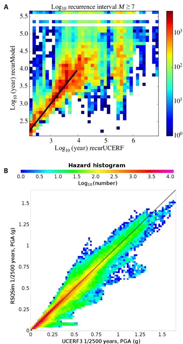
Fig. 1. Hazard-relevant measures in the simulator compared with the UCERF3 hazard model. (A) Recurrence intervals in the earthquake simulator compared with the UCERF3 hazard model. Plot shows a two-dimensional (2D) pointwise histogram of 265k elements on fault for M \geq 7 . Color shows number in histogram. The diagonal solid black line shows what would be perfect agreement. The lower left part shows the fastest-moving areas of the fault system with the shortest recurrence intervals. The horizontal lines at the top show the finiteness of the catalog, with the top horizontal set being patches that have broken once during the catalog above the cutoff magnitude, the next horizontal set below having broken twice, and so on. (B) Pointwise shaking hazard in the simulator compared with UCERF3. This is for a standard hazard measure, 2% in 50 years peak ground acceleration (PGA). Plot shows 2D pointwise shaking hazard across California coming from M 6.5+ events for the simulator events compared with on-fault UCERF3 events. Note that the hazard measure agrees even better than the recurrence intervals.
