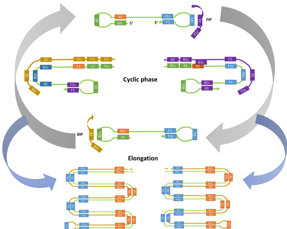
Fig. 3 Second and third step of LAMP: the cyclic amplification and elongation leading to strand displacement DNA synthesis. Modified from (Bruce, Leterme et al. 2015).
