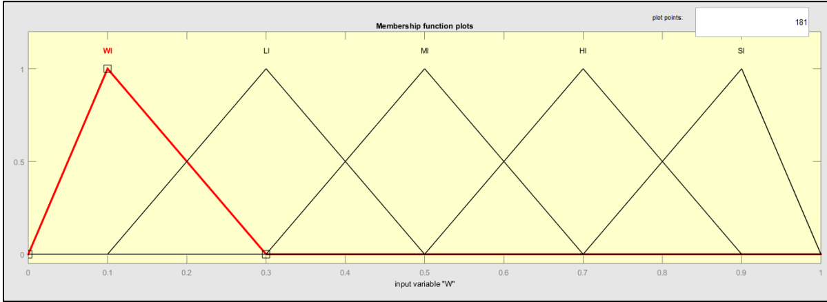
Figure 2: Triangular Membership Function
