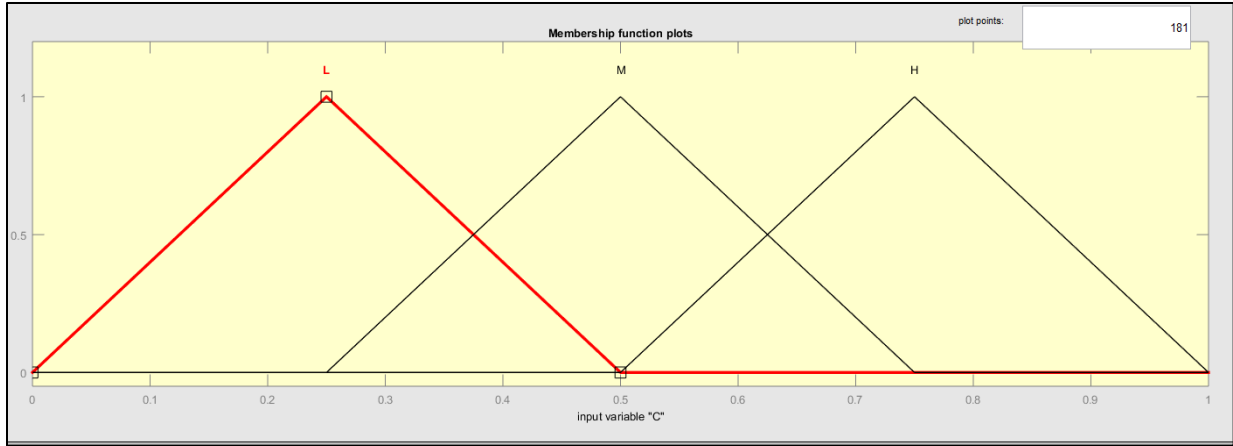
Figure 3: Triangular Membership Function
