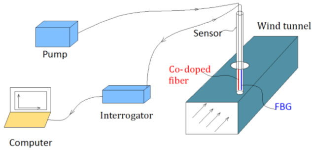
Fig. 3 Schematic of the fiber-optic 'hot-wire' sensing system showing the laser pump, the demodulator/FBG interrogation system, the probe placed in a wind tunnel for testing and evaluation and the computer where the outputs are visualized
