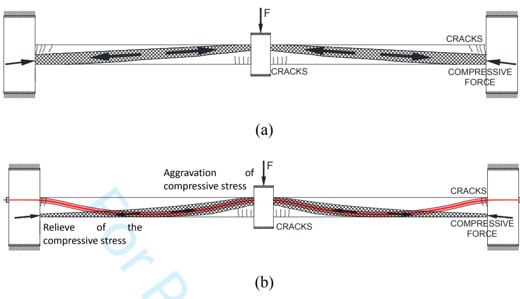
Fig. 5– Schematic of the compressive arch action: (a) RC specimen; (b) PC specimen
