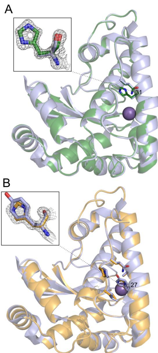
Figure 6. Superposition of SpMnSOD1 wild type with mutants A31H (A) and Y27H (B).
