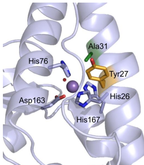
Figure 5. Location of amino acid replacements found in Spingobacterium sp. MnSOD1.
