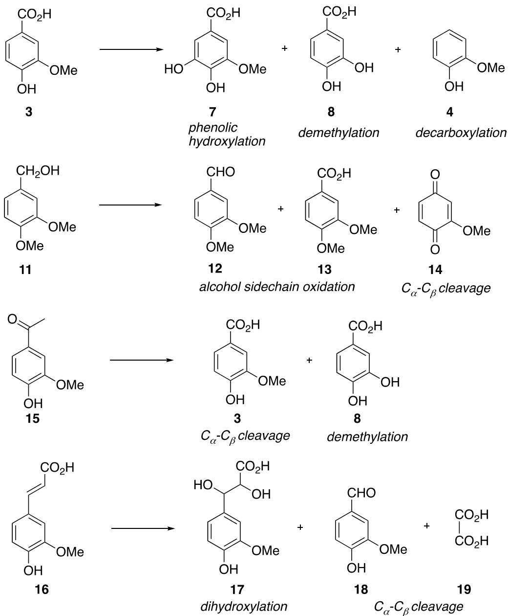
Figure 2. Transformation of monomeric aromatic substrates by SpMnSOD1
