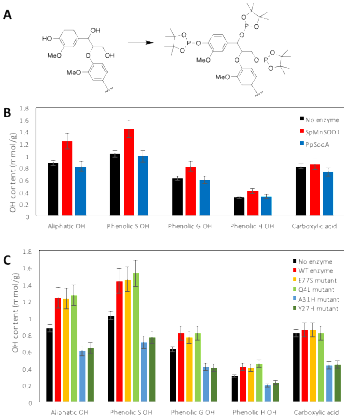
Figure 4. Changes in lignin OH content after treatment by SpMnSOD1
