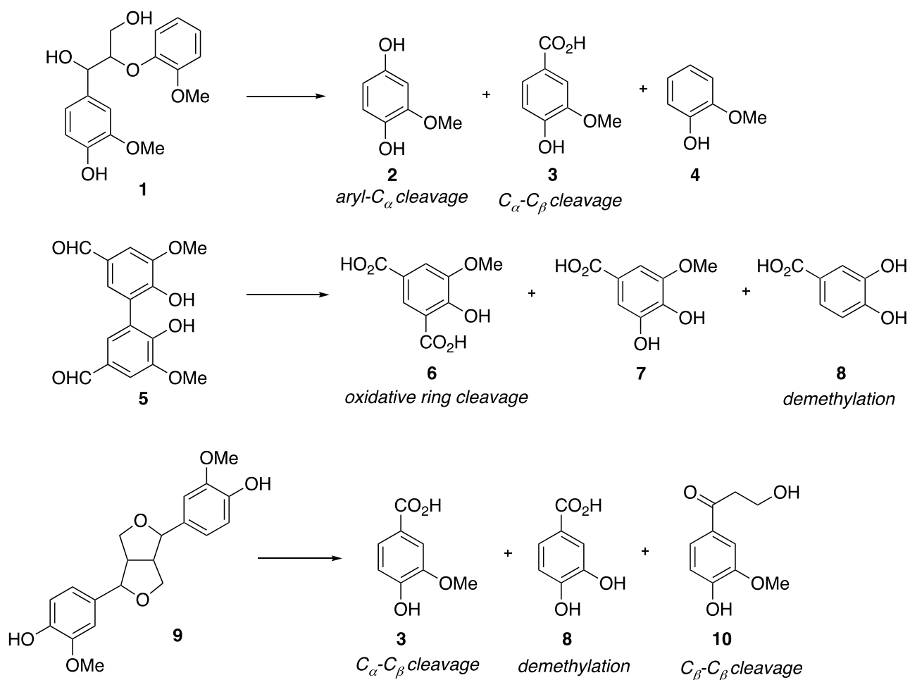
Figure 1. Transformation of dimeric lignin model compounds by SpMnSOD1
