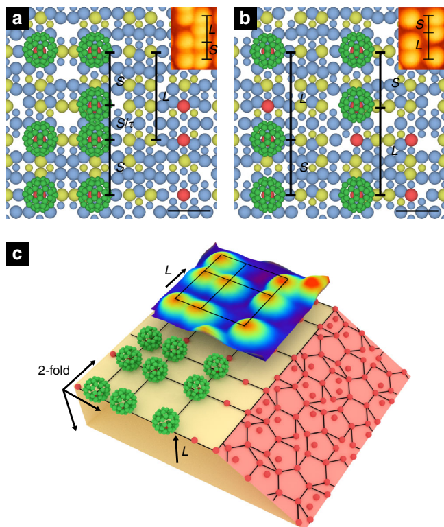
Fig. 3 Adsorption sites. a, b Comparison between C 60 motifs observed by scanning tunnelling microscopy (STM) and the model structure of icosahedral ( i )-Al-Pd-Mn. Model structures showing C 60 adsorbed atop Mn atoms, forming S \times S and S \times L tiles. Two images are taken from two different sections of the surface plane in order to illustrate common STM features. The insets in a, b are sections of the STM image from Fig. 1c. The inset in a shows an additional C 60 adsorbed at a \tau -deflated position, which appears as a squashed (i.e., non-circular) molecule. Al = blue, Pd = yellow, Mn = red and C 60 = green. Atoms in different layers are presented in different sizes, with the largest in the top layer. Scale bars in a, b represent 1 nm. c A block of the model structure of i -Al-Pd-Mn displaying five-fold (pink) and two-fold (cream) planes, with C 60 adsorbed atop Mn atoms. The orientation of C 60 is arbitrary. Only Mn atoms are shown for clarity. There are three equivalent two-fold axes in icosahedral quasicrystal, which are orthogonal to each other: two of them are in the surface plane and the third is perpendicular to the surface plane. These directions are indicated by arrows. An STM image is superimposed for comparison
