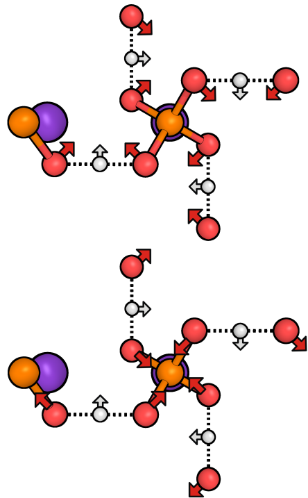
Figure 9: Schematic top views of the atomic displacements for the A_1 optical modes of the PE phase that couple significantly to the FE one: the strong coupled IMB mode at 543 \text{ cm}^{-1} (top panel) and the weak coupled mode at 917 \text{ cm}^{-1} (bottom panel). H atoms: white spheres, O atoms: red spheres, P atoms: orange spheres, and K atoms: violet spheres (see also the corresponding labels in Fig. 3).
