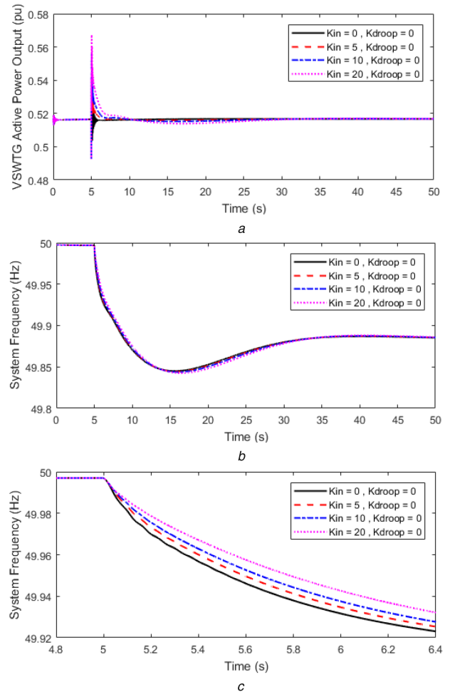
Fig. 4 Impact of emulated inertia controller
