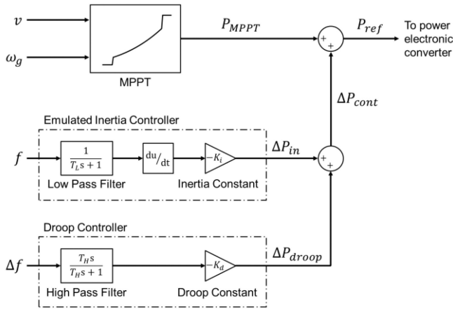
Fig. 2 Frequency response system based on [4]
