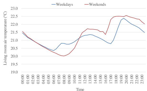
Figure 2 Weekday and weekend living room indoor air temperature profiles in DW05 during the heating season
