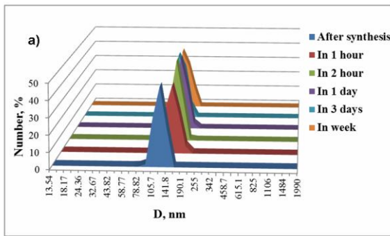
Fig.9. Changes in particle size distributions of three-layered capsules with time at pH 7 (a), pH 9.2 (b).
