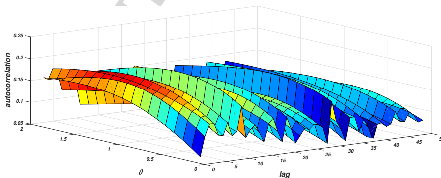
Figure 4: Taylor Effect
