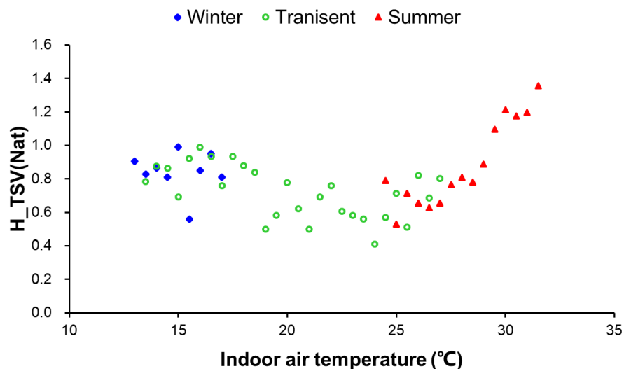
Fig. 4. Relationship between entropy of TSV and indoor air temperature
