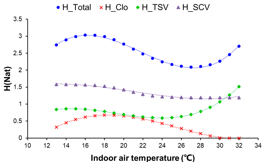
Fig. 7. The regression models of the information entropy of Clo, TSV, SCV and Total
