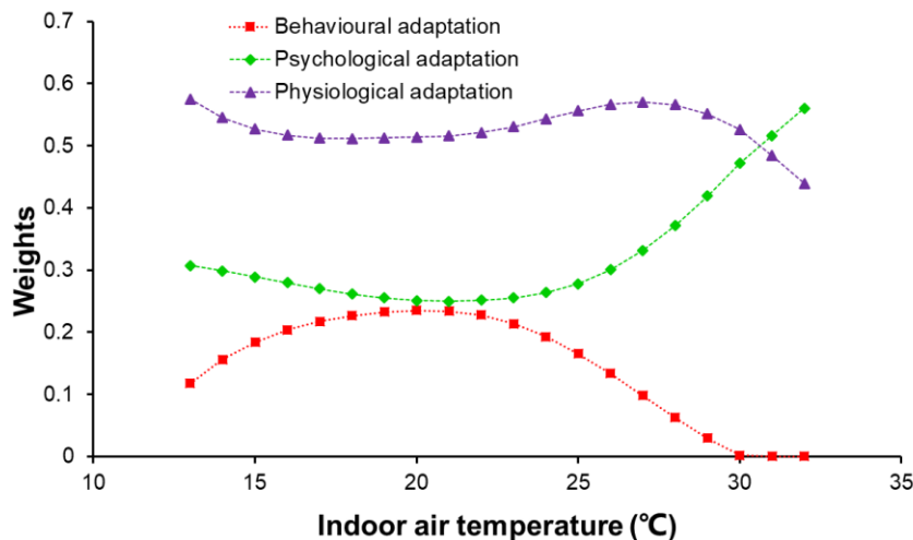
Fig. 9. The relationship between the weights of three categories of adaptation and indoor air temperature.
