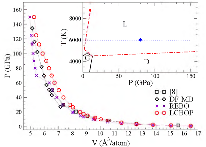
FIG. 1: (Color online) Equation of state of liquid carbon at T=6000\text{K} . The inset shows the P-T phase diagram, with diamond (D), graphite (G) and liquid (L) domains: the dotted curve is the sampled isotherm; the solid curves are experimental data: the diamond-graphite coexistence curve from Bundy 11 , the graphite melting curve from Togaya 12 . The dot-dashed line is the estimated diamond melting line from Glosli and Ree 13 , obtained with Brenner potential; the dashed curves are the liquid-liquid coexistence curve ending in a critical point and its graphite melting curve from Glosli and Ree 7 . The solid \diamond in the inset indicates the switching in coordination shown in Fig. 2.
