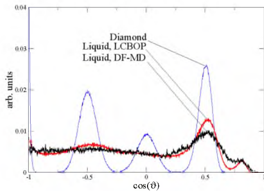
FIG. 5: (Color online) Angular correlation functions for second neighbors (see text) with state parameters as in Fig. 3. The peaks for the diamond are spread around the theoretical values for an fcc lattice of -1, -0.5, 0, 0.5, with weights 6/66, 24/66, 12/66, 24/66.
