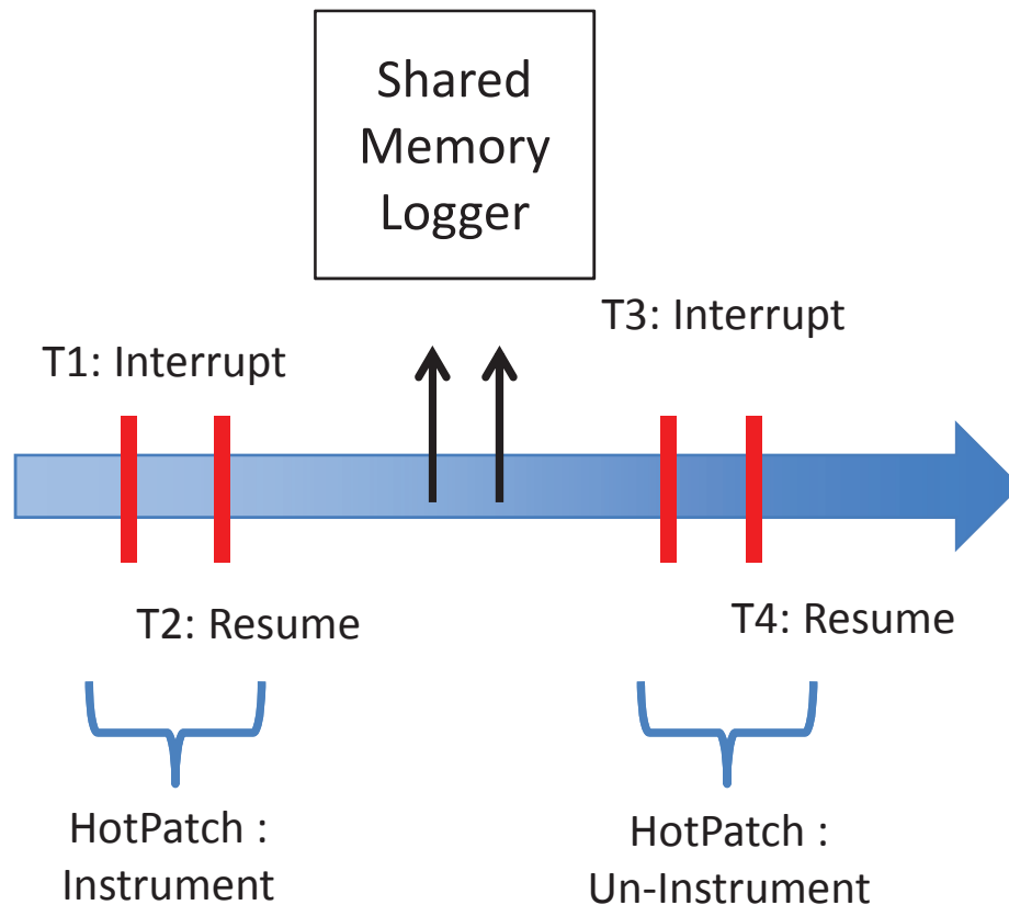
Figure 5.3: HotPatching Workflow.
