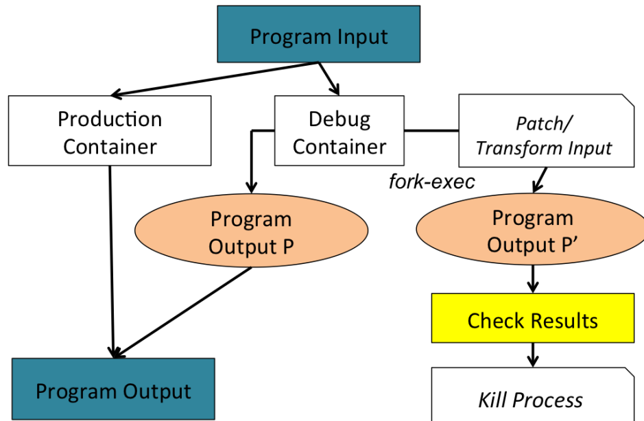
Figure A.2: Debugging Strategies for Active Debugging
