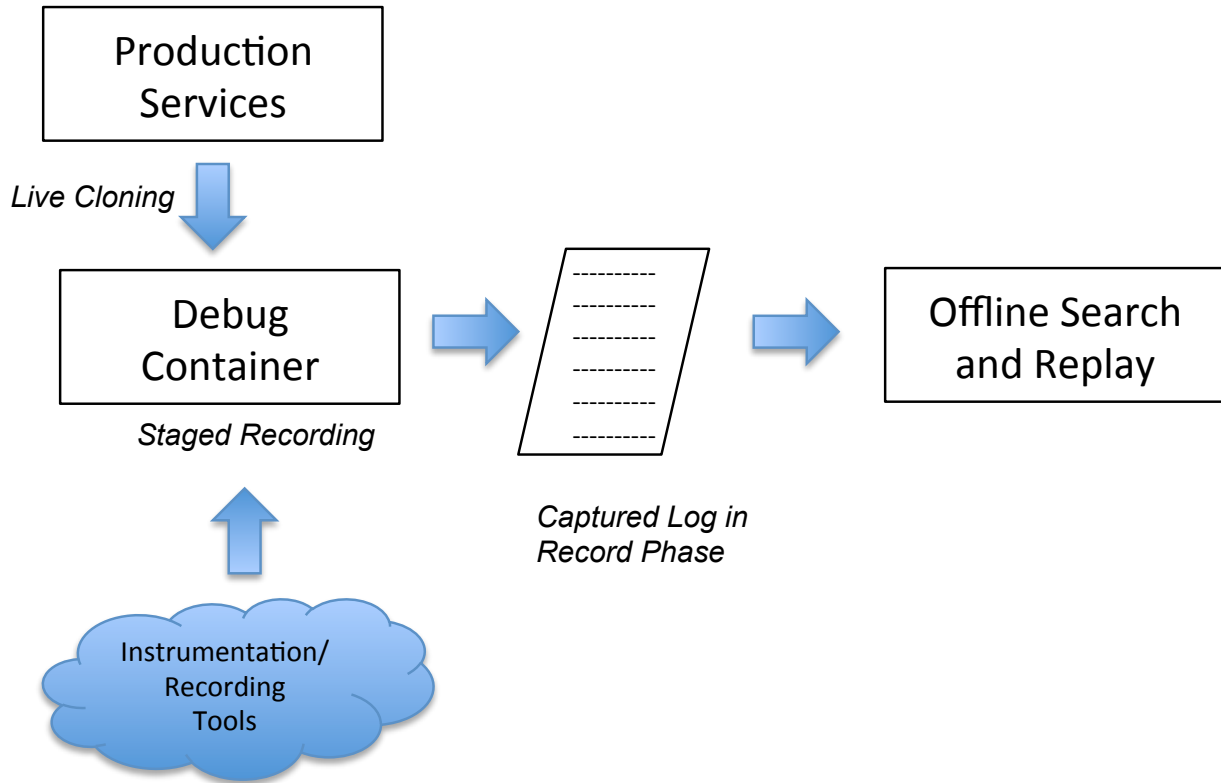
Figure 6.1: Staged Record and Replay using Parikshan
