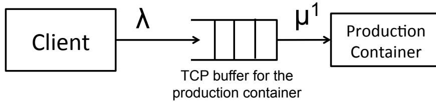
Figure 6.3: Parikshan applied to a mid-tier service
