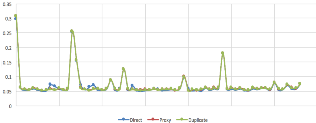
Figure 3.8: Latencies in all different modes for wikipedia trace
