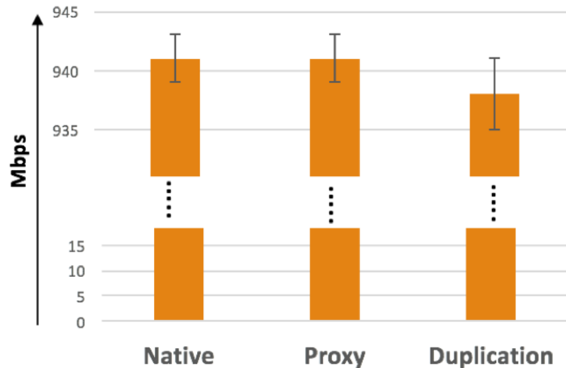
Figure 3.7: Performance impact on network bandwidth when using network duplication. The above chart shows network bandwidth performance comparison of native execution, with proxy
