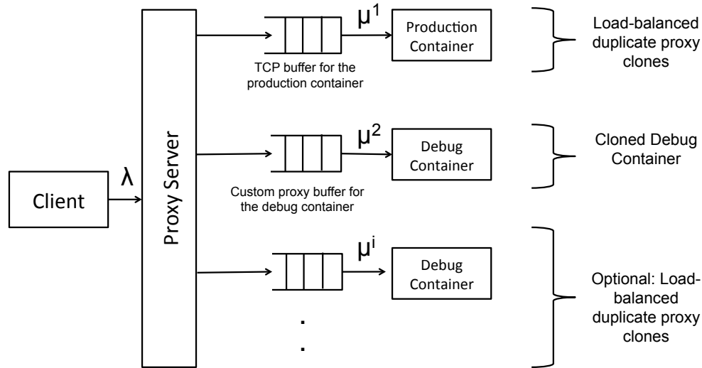
Figure 6.5: This figure shows how queuing theory can be extended to a load balanced debugging scenario. Here each of the debug container receive the requests at rate \lambda , and the total instrumentation is balanced across multiple debug containers.
