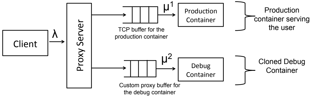
Figure 6.4: External and Internal Mode for live cloning: P1 is the production, and D1 is the debug container.
