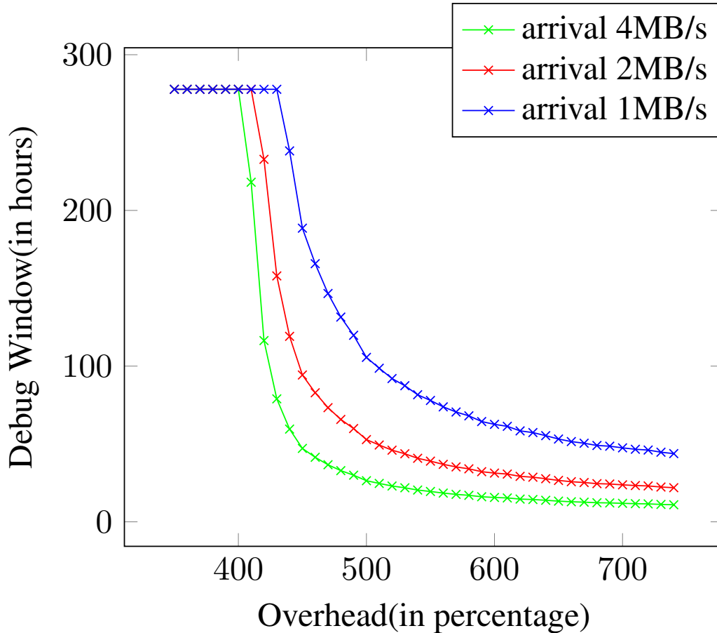
Figure 3.6: Simulation results for debug-window size. Each series has a constant arrival rate, and the buffer is kept at 64GB.
