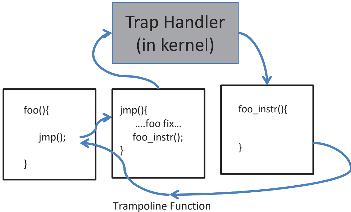
Figure 5.4: Traditional Trampoline based Dynamic Instrumentation Mechanisms.
