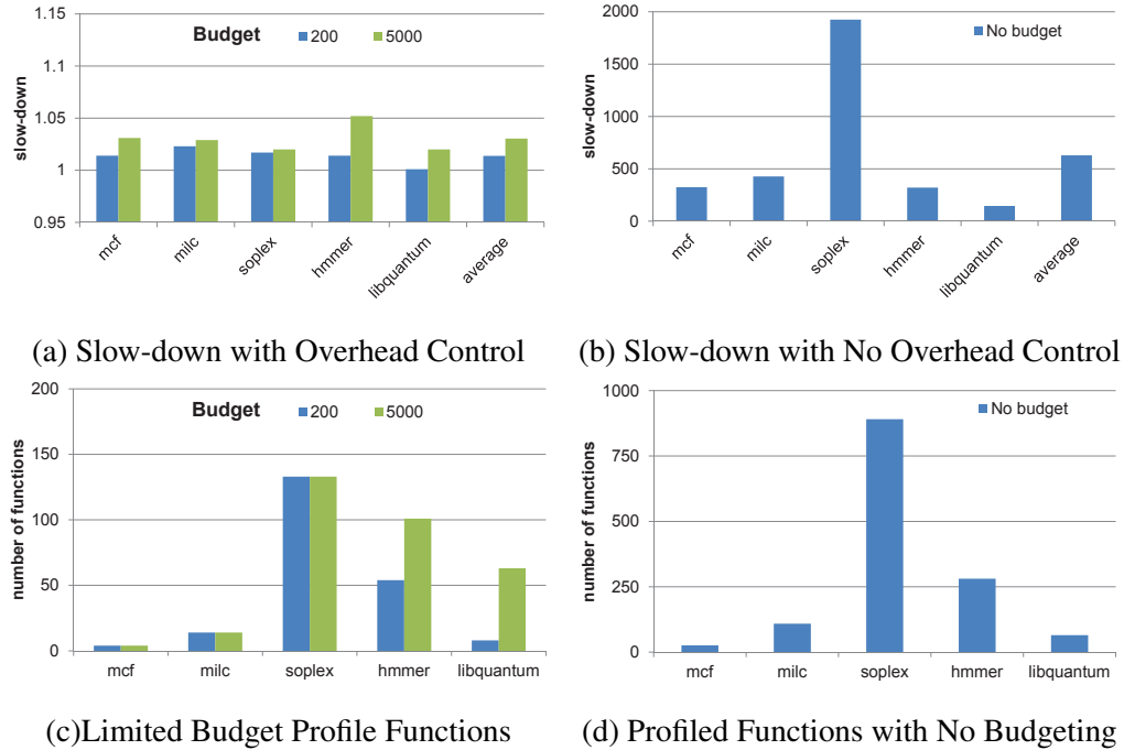
Figure 5.9: Overhead Control and Number of Captured Functions Comparison.
