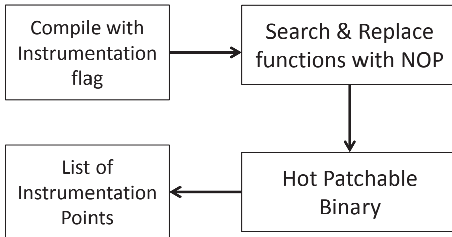
Figure 5.1: The Process of ColdPatching.
