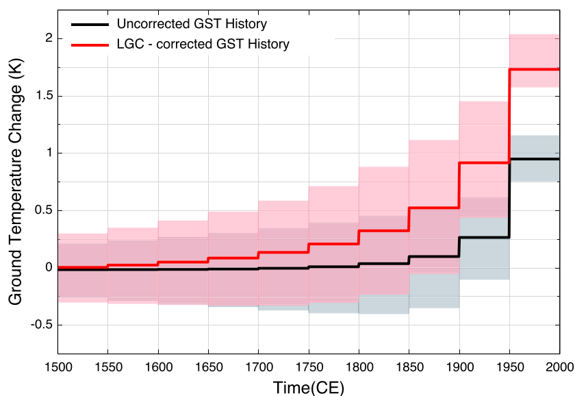
Figure 4. Mean GST history as departures from the long-term temperatures at each site for the IHFC borehole database over North America truncated at 300 m (259 borehole temperature profiles) retrieved from the uncorrected data (black line), and LGC-corrected data (red line). Shaded regions represent the uncertainty envelope estimated from the uncertainty from the determination of the semiequilibrium geothermal gradient and the long-term surface temperature for uncorrected (grey shade) and LGC-corrected (pink shade) data. The LGC-corrected uncertainty envelope also includes the additional uncertainties from the 75% GSM ensemble confidence intervals. Both GST histories are referenced to the quasi-equilibrium geothermal regime and its long-term past surface temperature.
