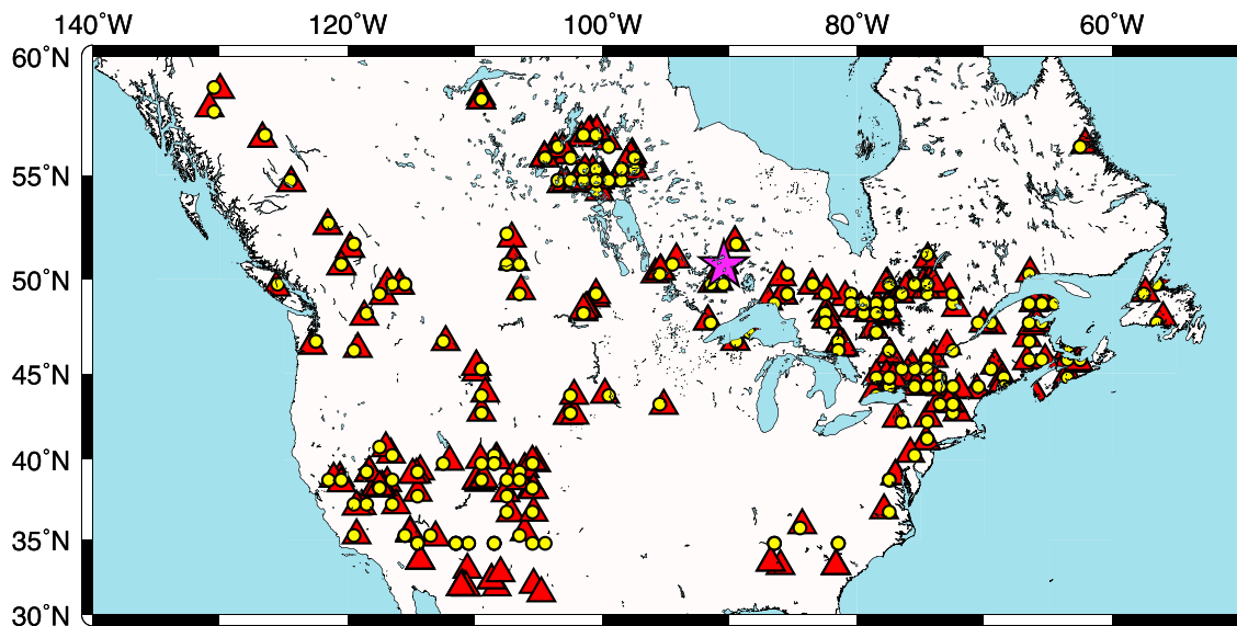
Figure 1. Simulation domain (140°W, 30°N); (52.5°W, 60°N) and grid cell locations within the GSM. Yellow circles mark the locations of the nearest grid cells from which simulated temperatures are used for borehole corrections. Red triangles mark the location of borehole temperature profiles from the IHFC database. The star marks the location of the Minchin Lake borehole temperature profile used as a detailed example in text.
