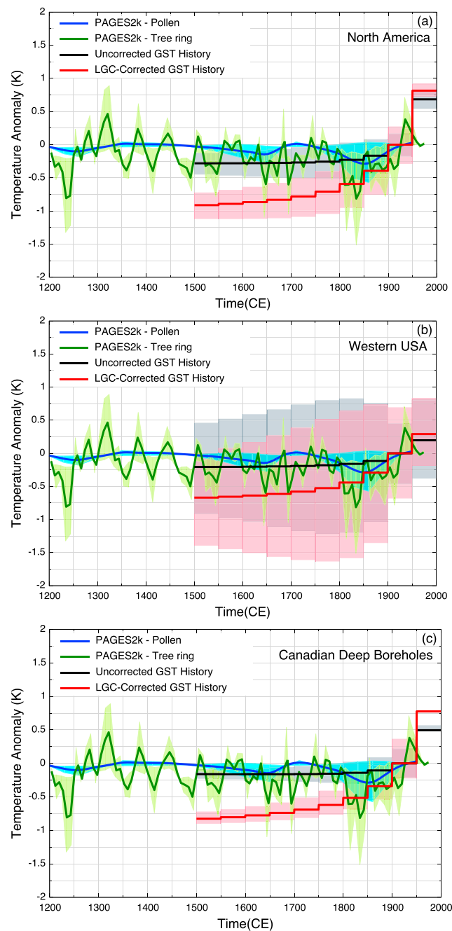
Figure 5. GST history reconstructions and proxy paleoclimatic reconstructions. Time series are expressed as departures from the 1900–1950 mean for (a) North America, (b) Western USA, and (c) Canadian Deep Boreholes. Shading represents 95% confidence range for each reconstruction. For uncorrected and LGC-corrected data, the uncertainty envelope is estimated from the uncertainties from the estimate of the semiequilibrium geothermal gradient and the long-term surface temperature for uncorrected (grey shade) and LGC-corrected (pink shade) data. The LGC-corrected uncertainty envelope also includes the uncertainties from the 75% GSM ensemble confidence intervals.
