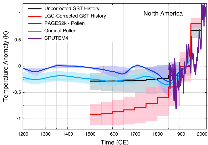
Figure 6. GST history reconstructions compared to pollen mean July temperature reconstructions and the North American SAT annual record from meteorological data. Time series are expressed as departures from the 1900–1950 C.E. interval. The original pollen data has been scaled to match the 1850–1900 to 1901–1950 mean shift in the CRU meteorological data.
