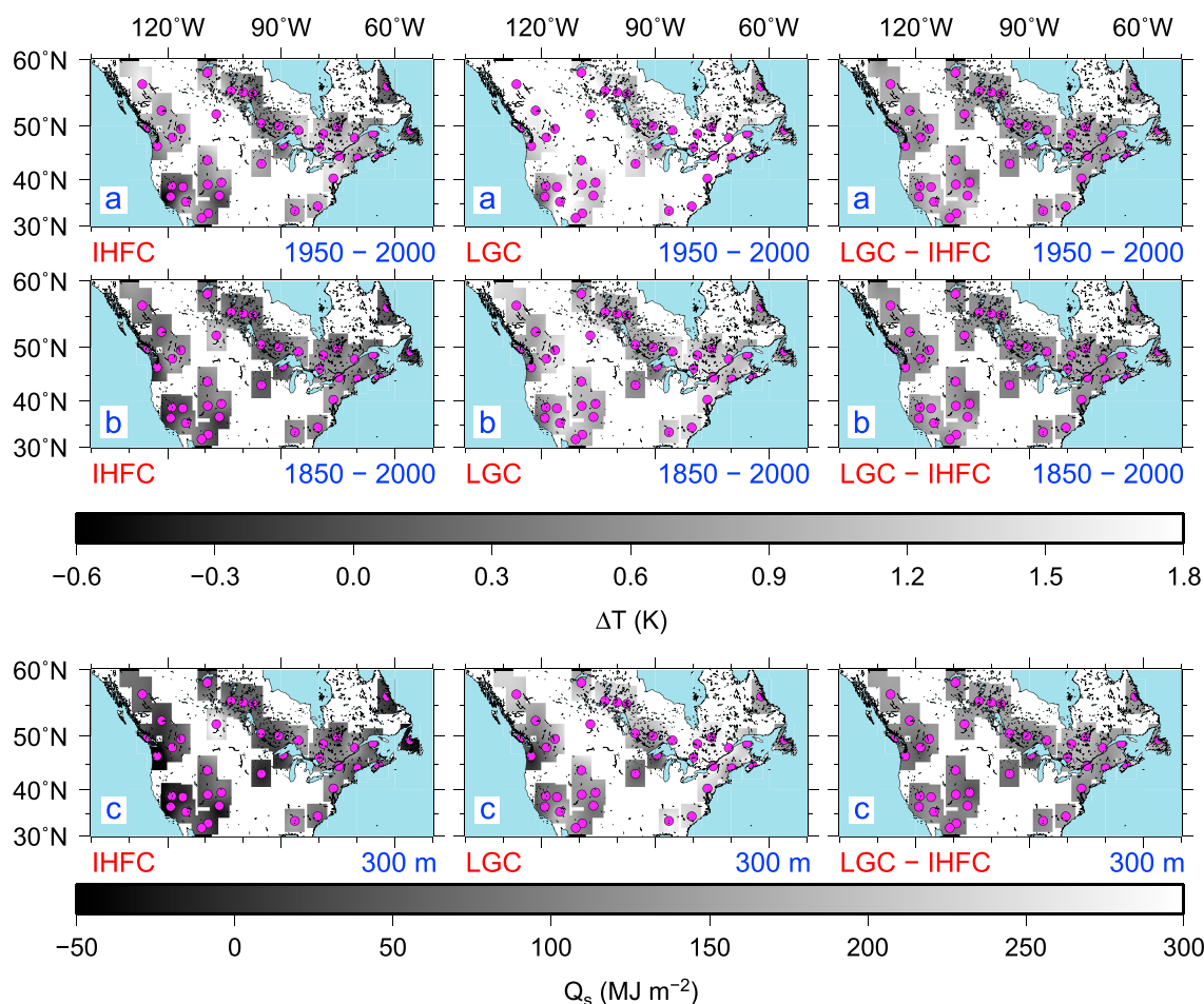
Figure 3. GST history for the IHFC data truncated to 300 m for (a) GST changes from 1950 to 2000, (b) GST changes from 1850 to 2000, and (c) subsurface heat storage for the same data. The left column corresponds to the original data, middle column to the LGC-corrected data, and the right column shows the results for the respective differences (LGC-corrected—IHFC data). See Figure S2 in the supporting information for a different (color) version of this figure.
