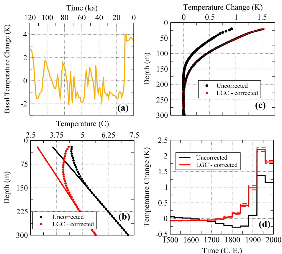
Figure 2. Example of the correction procedure using the borehole temperature profile for Minchin Lake, Canada ( -90.480^{\circ} , 50.710^{\circ} ). (a) Ice sheet basal temperature history for 120 ka from GSM for the model grid point closest to Minchin Lake, (b) Black dots represent the measured borehole temperature profile, while red dots represent the LGC-corrected data. Black and red lines represent the estimated quasi-equilibrium geothermal profiles for this site before and after corrections, respectively. (c) Subsurface temperature anomalies and their 75% confidence levels estimated for the original (black) and LGC-corrected data (red); (d) GST history estimated from the original data (black) and corrected data (red) along with their 75% confidence levels. The uncertainties for the uncorrected data have been examined in detail in Beltrami et al. [2015a].
