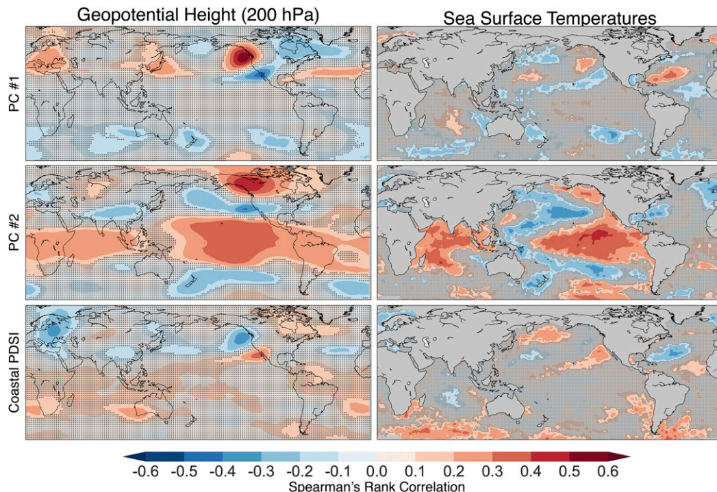
FIG. 10. Point-by-point correlations (Spearman's rank) for the ClimGrid PCs and coastal PDSI vs October–March (left) 200-hPa geopotential heights from the Twentieth Century Reanalysis (1896–2014) and (right) SSTs from HadISST (1896–2016). Insignificant correlations ( \rho > 0.10 ) are stippled in gray.
