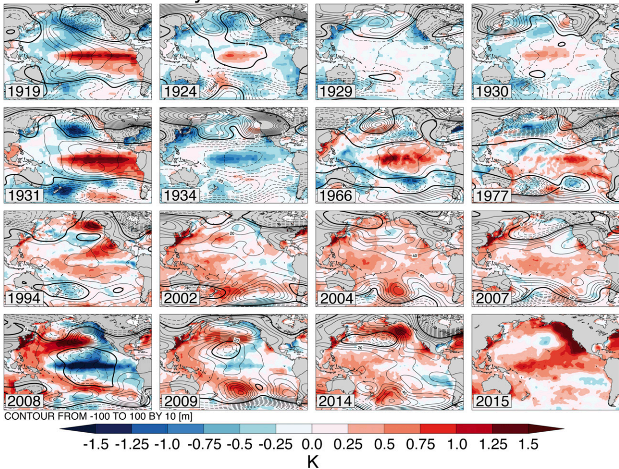
FIG. 11. For each coastal drought event, October–May average anomalies in 200-hPa geopotential height (contours, m) and SSTs (shading, K). Because the Twentieth Century Reanalysis ends in 2014, height anomalies for the 2015 event were not available.
