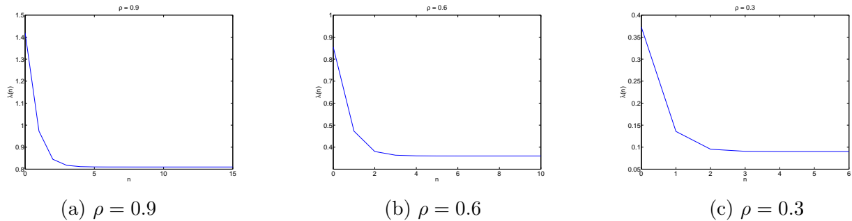
Figure 4: Illustrating the convergence of conditional arrival rates, \lambda(n) , for a given queue of an M/M/K/JSQ/PS , with mean job size 1, where K = 2 .
