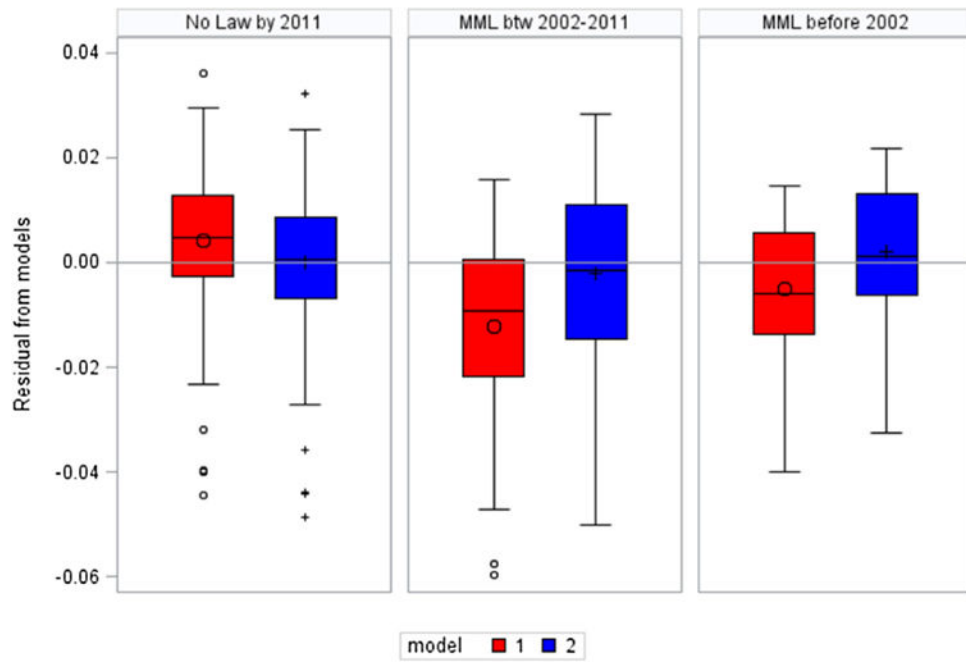
Residuals from fitted Models to NSDUH state MJ use among 12-17 year olds from 2002/3 - 2010/11
