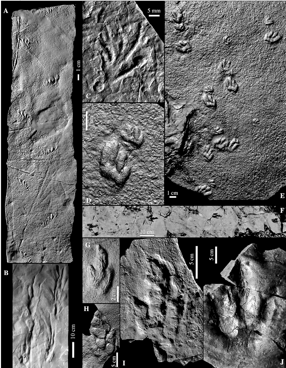
Figure 35: Post-ETE (latest Rhaetian) reptile footprints from the uppermost Passaic Formation at Stop 1.7: A, C, Rhynchosauroides n. sp.; B, swimming brontoozid tracks; D-E, Batrachopus deweyii ; F, trackway of medium-sized brontoozid Anchisauripus sillimani ; G, smaller brontoozid Grallator sp.; H,
