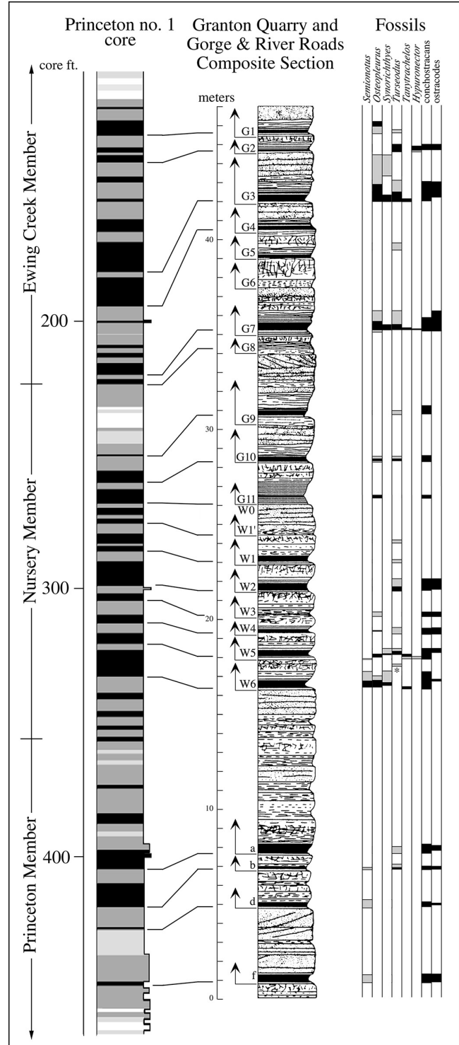
Figure 31: Composite section in vicinity of stop 1.2-1.5 with the distribution of fossils and correlation to the NBCP Princeton no. 1 core. Modified from Olsen (2003).
