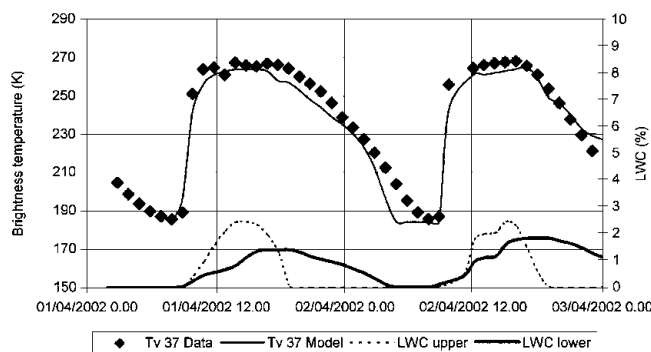
Fig. 10. Measured and simulated microwave brightness temperature T_b at 37 GHz, vertical polarization, as a function of time. Lower lines represent simulated LWC of the upper and lower layers respectively, used as inputs to the electromagnetic model. Dates are day/month/year.
