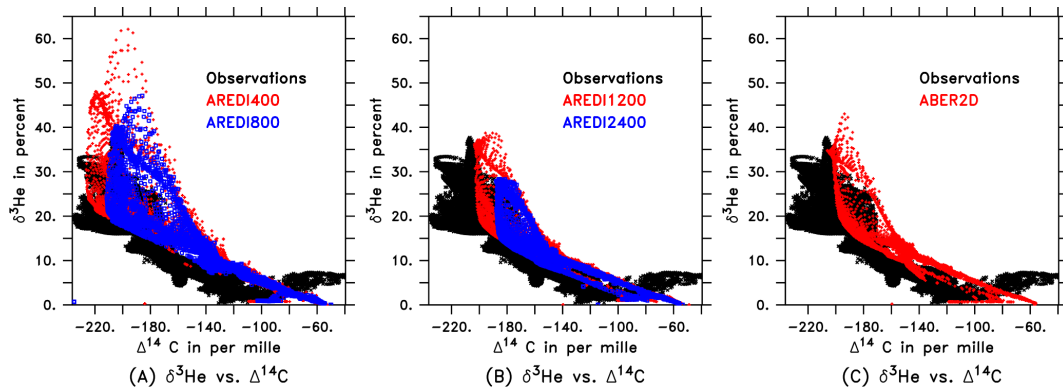
Figure 7. Scatterplots of \delta^3\text{He} vs. \Delta^{14}\text{C} for different values of A_{\text{Redi}} . On all plots observations are in black. (a) AREDI400 (red) and AREDI800 (blue). (b) AREDI1200 (red) and AREDI2400 (blue) (c) ABER2D (red).
