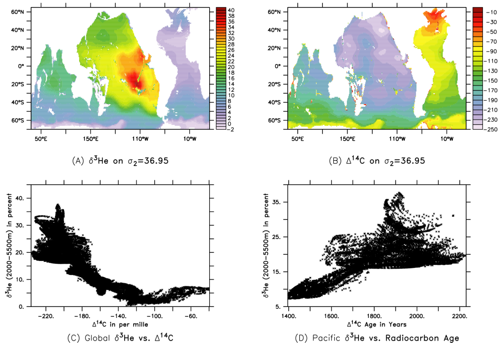
Figure 1. \delta^3\text{He} and radiocarbon in the ocean. (a) \delta^3\text{He} from Bianchi et al. (2010) on \sigma_2 (potential density relative to 2000 m minus 1000\text{ kg m}^{-3} ) of 36.95. (b) \Delta^{14}\text{C} on \sigma_2 = 36.95 from Key et al. (2004). (c) Vertically averaged \delta^3\text{He} vs. vertically averaged \Delta^{14}\text{C} (2000–5500 m). (d) Vertically averaged \delta^3\text{He} vs. radiocarbon age, 2000–5500 m, Pacific sector only.
