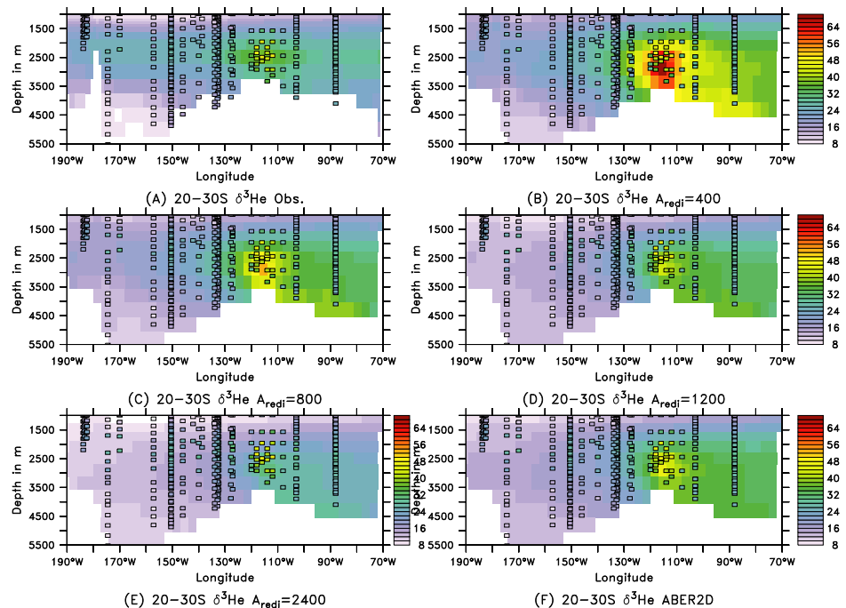
Figure 10. \delta^3\text{He} (in %) in the SE Pacific between the latitudes of 20 and 30° S. Symbols are taken from the observational data set of Bianchi et al. (2010). (a) Gridded data set of Bianchi et al. (2010) showing effects of smoothing. (b) AREDI400. (c) AREDI800. (d) AREDI1200. (e) AREDI2400. (f) ABER2D.
