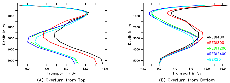
Figure 8. Overturning in the South Pacific at a latitude of 30^\circ\text{S} across the different model runs. Overturning is computed as a running sum of northward transport. (a) Overturning summed from top to bottom, emphasizing similarity in northward surface flow. (b) Overturning summed from bottom to top, emphasizing similarity in deep inflow of Antarctic Bottom Water.
