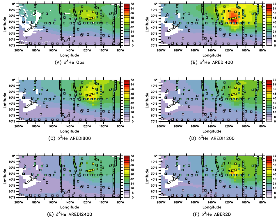
Figure 9. \delta^3\text{He} (in %) in the SE Pacific between the depths of 2250 and 2750 m. Symbols are taken from observational data set of Bianchi et al. (2010). (a) Gridded data set of Bianchi et al. (2010) showing effects of smoothing. (b) AREDI400. (c) AREDI800. (d) AREDI1200. (e) AREDI2400. (f) ABER2D.
