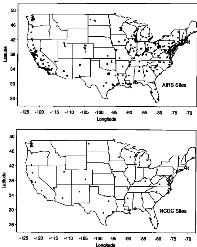
Figure 1. Ozone (EPA/AIRS) and temperature (NCDC) sites used in the trend analysis.
