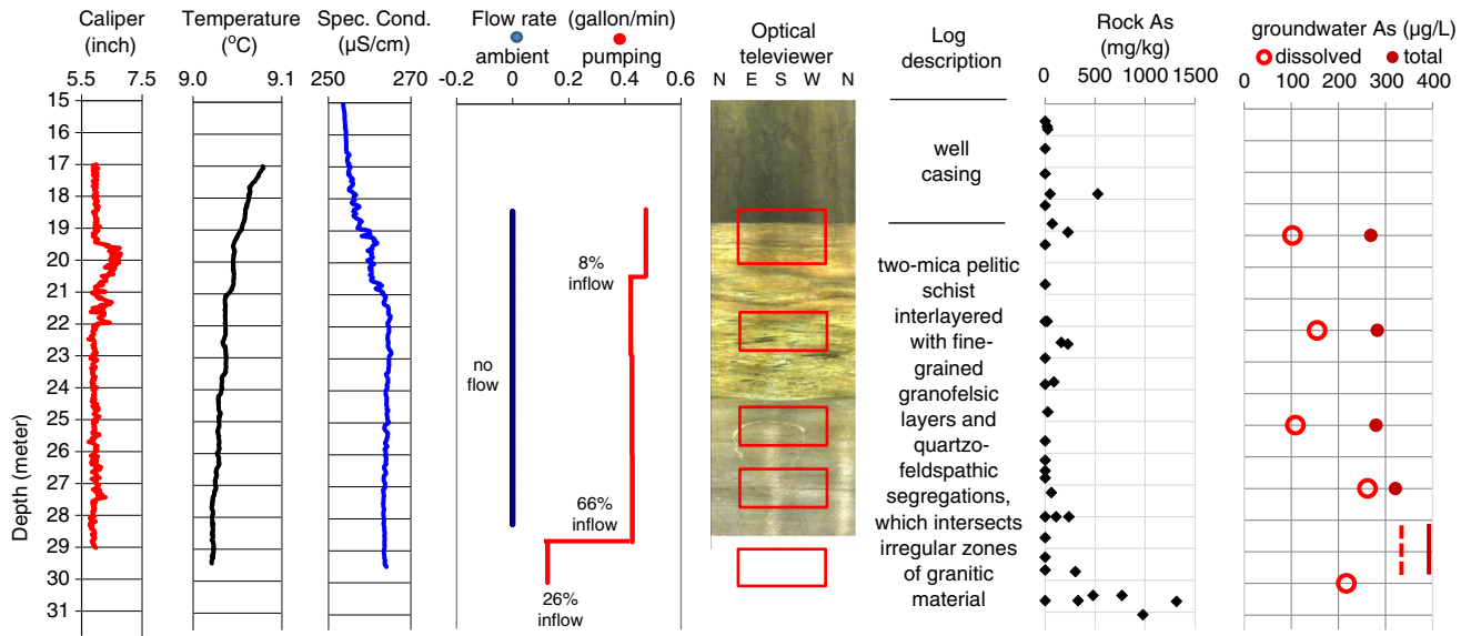
Fig. 4. Composite logs of caliper, water temperature, specific conductance, heat-pulse flow meter, optical televiewer, core description, rock arsenic concentrations, and fracture water arsenic concentrations in well MA70190 in Litchfield, Maine. * Red squares indicate the sampling intervals for fracture specific water. * Groundwater [As] at the end of pumping test: dash line – dissolved [As], solid line – total [As]. (For interpretation of the references to color in this figure legend, the reader is referred to the web version of this article.)
