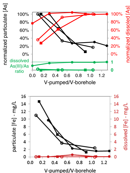
Fig. 6. Borehole water arsenic (normalized to the maximum concentrations) and dissolved As(III)/As ratio (top), and iron concentrations (bottom) during pumping tests in wells MA70076 (solid square), MA70138 (open circle), and MA70190 (solid circle).
