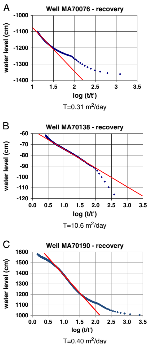
Fig. 5. Cooper–Jacob straight-line method to estimate borehole transmissivity of wells MA70076 (A), MA70138 (B), and MA70190 (C).
