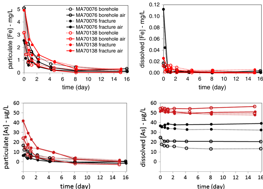
Fig. 7. Arsenic and iron concentrations in cubitainer experiments.
