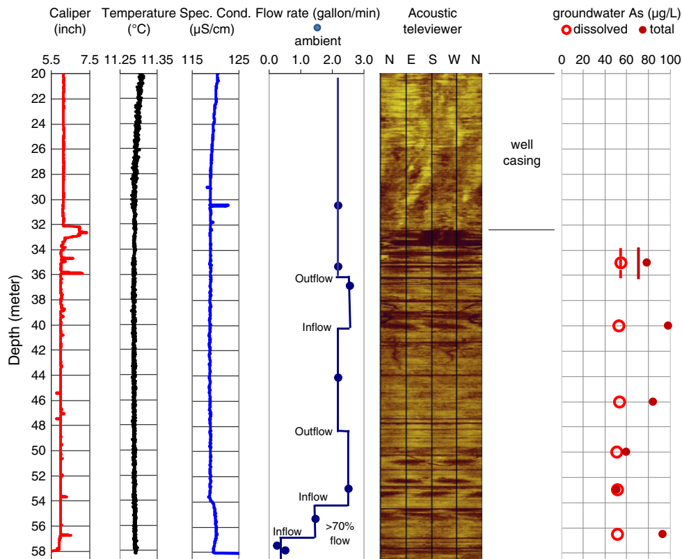
Fig. 3. Composite logs of caliper, water temperature, specific conductance, heat-pulse flow meter, acoustic televiewer, and fracture water arsenic concentrations in well MA70138 in Manchester, Maine. * Groundwater [As] at the end of pumping test: dash line – dissolved [As], solid line – total [As].
