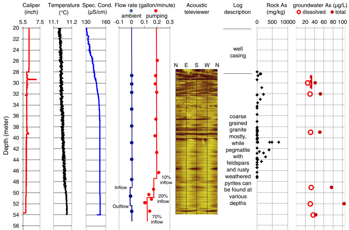
Fig. 2. Composite logs of caliper, water temperature, specific conductance, heat-pulse flow meter, acoustic televiewer, core description, rock arsenic concentrations, and fracture water arsenic concentrations in well MA70076 in Manchester, Maine. * Groundwater [As] at the end of pumping test: dash line – dissolved [As], solid line – total [As].
