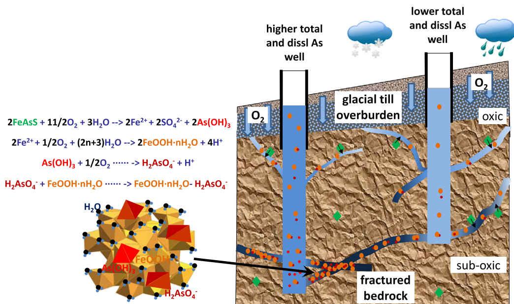
Fig. 8. A schematic graph (right) and geochemical processes (left) of arsenic evolution along groundwater flow paths in fractured bedrock aquifers in central Maine. * The intensity of blue colors reflects the redox conditions, with light blue indicating more oxic and dark blue more sub-oxic. (For interpretation of the references to color in this figure legend, the reader is referred to the web version of this article.)
