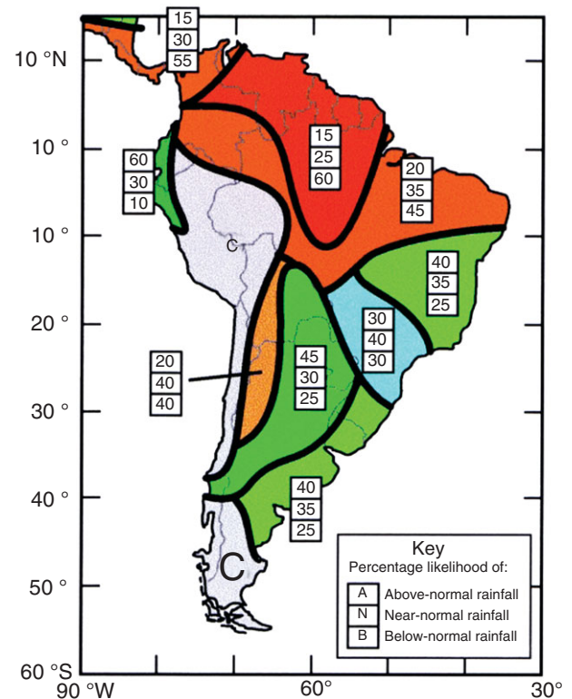
FIGURE 2 | IRI probabilistic seasonal forecast for January–March 1998 precipitation, produced in January 1998. The figure depicts for each of the colored zones the probability (in percent) of above-normal (upper box), near-normal (center box), and below-normal (lower box) precipitation for the season January–March 1998, as defined by terciles of the climatological distribution of rainfall for those regions and season. ‘Red’ colors refer to regions where below-normal precipitation is most probable, and ‘green’ colors refer to regions where above-normal precipitation is most probable.
