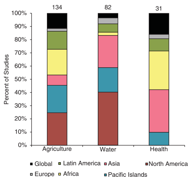
FIGURE 3 | Distribution of research articles addressing El Niño-Southern Oscillation (ENSO) forecast use, by sector and region. The numbers on top of each column correspond to the total number of articles on each sector.
