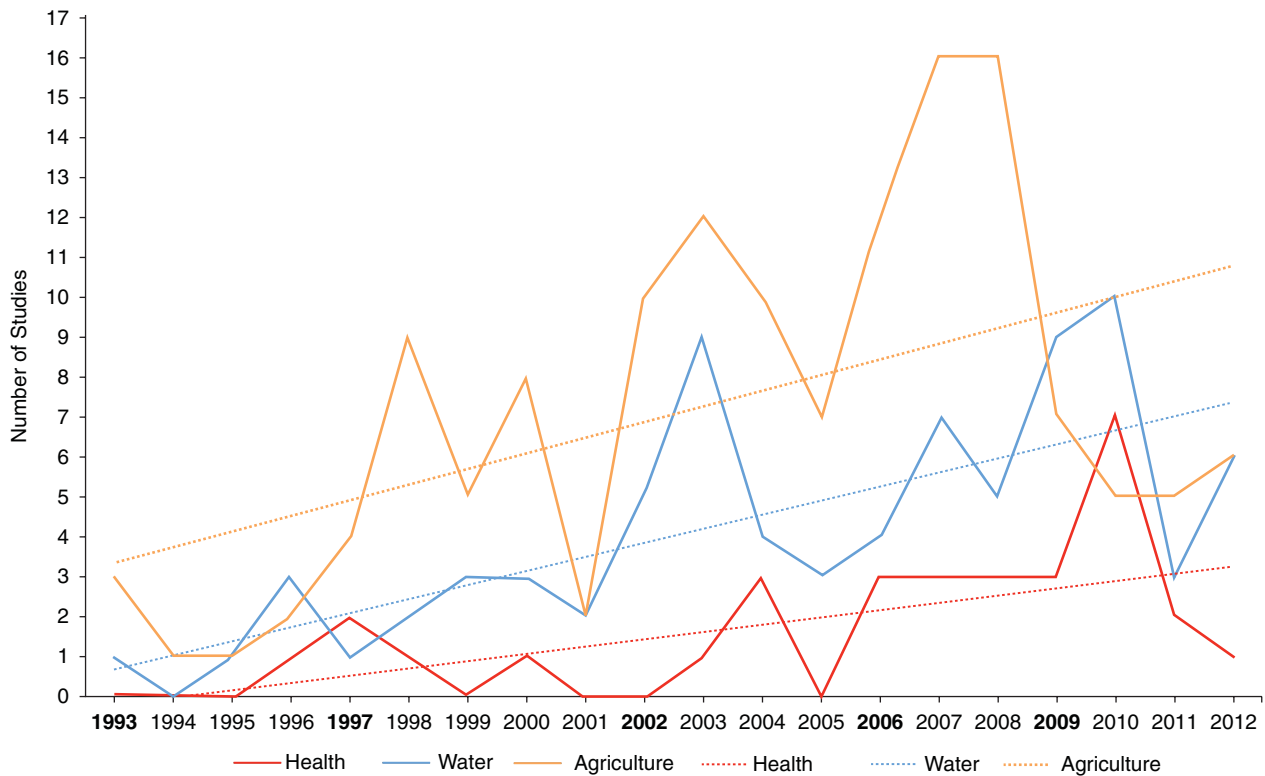
FIGURE 4 | Time evolution of the number of research articles addressing El Niño-Southern Oscillation (ENSO) forecast use. Solid lines show the actual time series for each sector, while the dotted lines sketch their long-term linear trend. El Niño years appear in bold in the x-axis.
