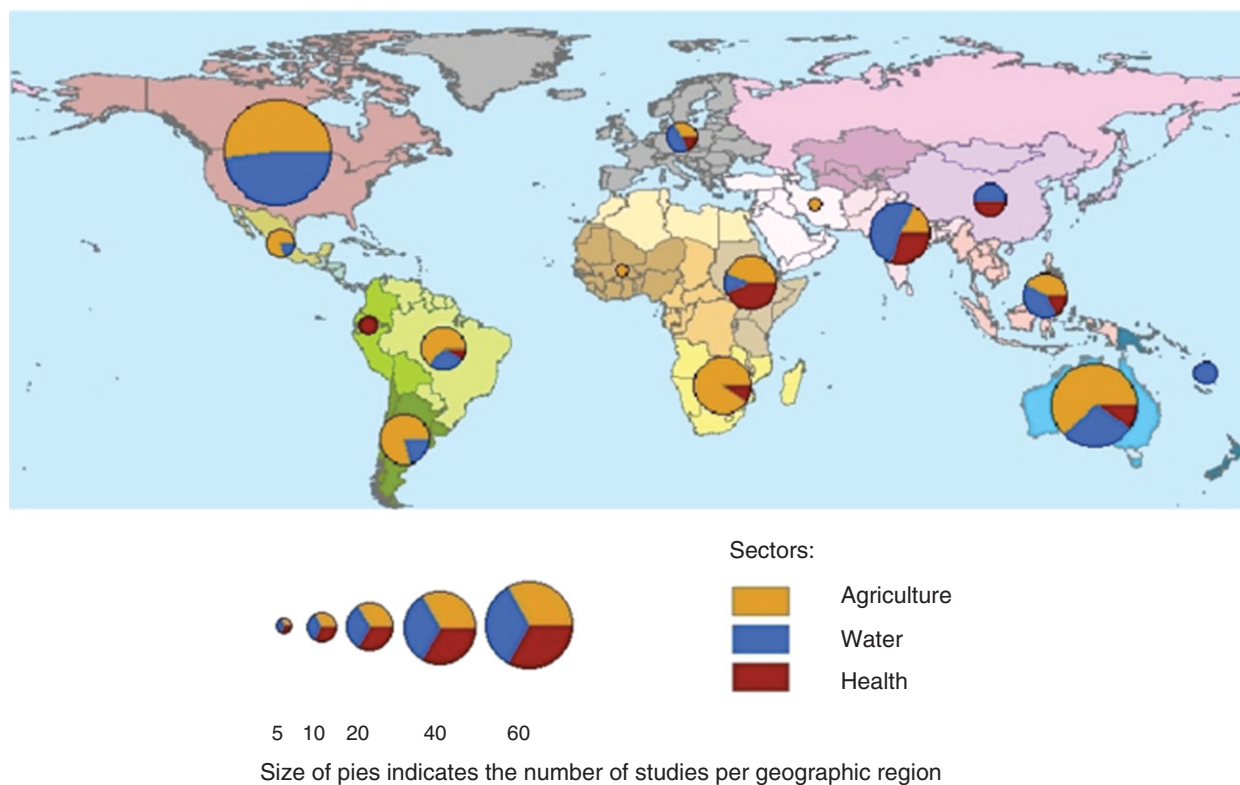
FIGURE 5 | Spatial distribution of research articles addressing El Niño-Southern Oscillation (ENSO) forecast use. The size of the pies is proportional to the number of studies. Regions are indicated on the map by background color.
