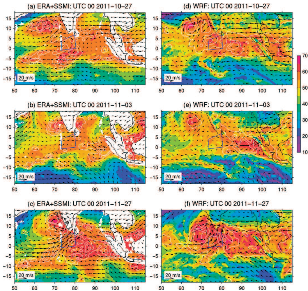
FIG. 8. (left) Total precipitable water from TMI and SSM/I (shaded), TRMM daily precipitation (white; 10, 30, and 50 mm day -1 ), and ERA-Interim horizontal winds at 850 hPa (vectors). (right) As in (left), but for the WRF simulation. Three time snapshots are shown: (top) 0000 UTC 27 Oct, (middle) 0000 UTC 3 Nov, and (bottom) 0000 UTC 27 Nov.
