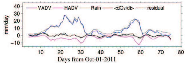
FIG. 13. Column-integrated water vapor budget over the NSA regions ( 0^{\circ} – 5^{\circ} N, 73^{\circ} – 80^{\circ} E): vertical advection (blue), horizontal advection (magenta), rain (gray), residual of the rhs of Eq. (1) (dotted), and the tendency term (black). A 3-day moving average is applied to all the time series.
