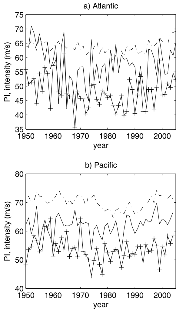
Figure 1. Time series of wind speed (crosses) and potential intensity (solid and dot-dash curves). Wind speed is computed by averaging the maximum intensities reached by all storms in a given year. Potential intensity is computed by averaging the values occurring at the first point on each track at which each storm reached its maximum intensity, over all storms for each year which reached at least hurricane intensity (solid curve). The dot-dash curve shows PI averaged over the main development region ( 10^{\circ} – 20^{\circ} N, 80^{\circ} – 20^{\circ} W for the Atlantic; 5^{\circ} – 25^{\circ} N, 100^{\circ} – 160^{\circ} E for the western North Pacific) and peak season (August–October for the Atlantic, July–October for the western North Pacific). Data for the (a) Atlantic and (b) western North Pacific.
