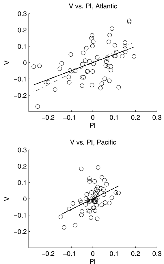
Figure 2. Scatter plots of wind speed and potential intensity. Wind speed is computed by averaging the maximum intensities reached by all storms in a given year, for those storms reaching at least hurricane intensity. Potential intensity is computed by averaging the values occurring at the first point on each track at which each storm reached its maximum intensity, over all storms for each year reaching at least hurricane intensity. Data for the (a) Atlantic and (b) western North Pacific. Both time series have been normalized and detrended, and have had their means removed. Least-squares regression lines computed from the data (solid curve) as well as the theoretical linear relationship (dot-dash curve) are also shown.
