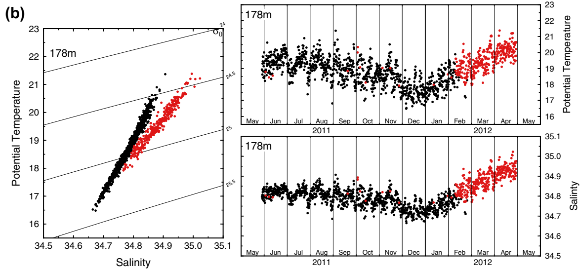
Figure 7b. Time series of potential temperature and salinity at TRBM 3, 121.7415°N, 15.8186°E, deployed 28 May 2011; recovered 30 April 2012. The red dots denote a saltier S-max, characteristic of the NEC tropical stratification.
