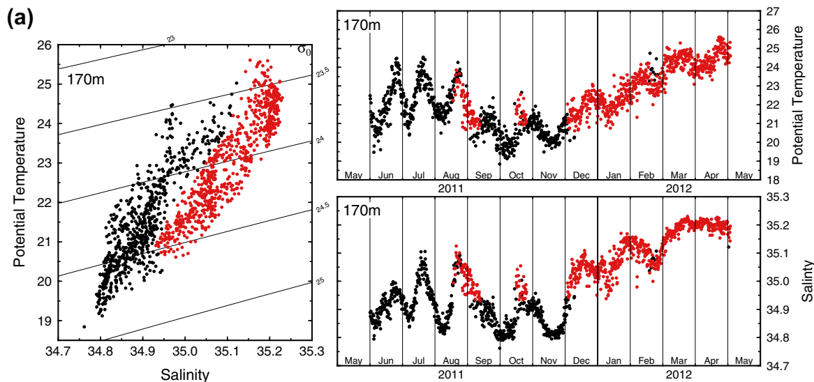
Figure 7a. Time series of potential temperature and salinity measured at the mooring 124.2274°N, 15.7540°E, at the southwest flank of Benham Bank, deployed 31 May 2011; recovered 4 May 2012. The red dots denote a saltier S-max, characteristic of the NEC tropical stratification.
