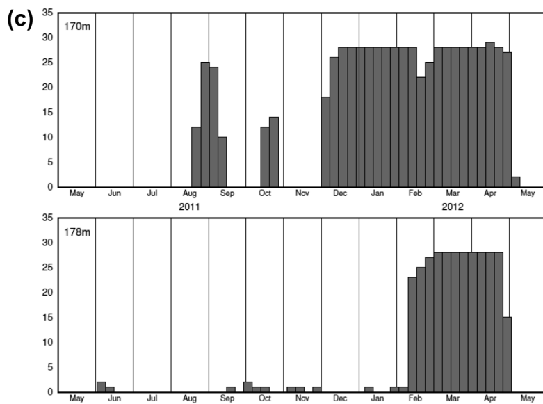
Figure 7c. Histogram of the number of red dots (marking the saltier NEC S-max) in 6 h block mean, for (top) the mooring at 124.2274°N, 15.7540°E and (bottom) the TRBM at 121.7415°N, 15.8186°E.
