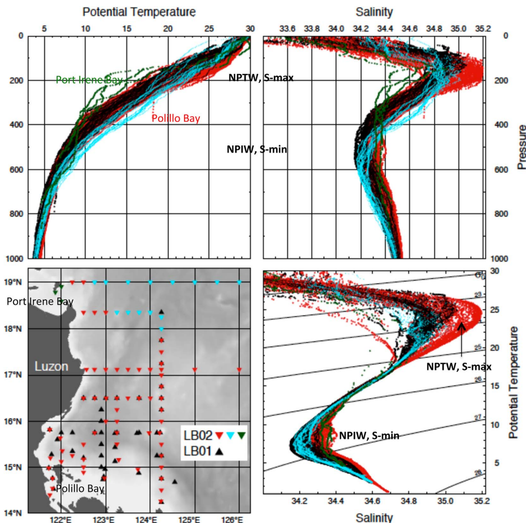
Figure 5. Lamoun Bay ship-based stratification. (top) Potential temperature (T) and salinity profiles versus pressure. (bottom right) T/S for the two cruises. (bottom left) Station map with different symbols denoting cruise. In 2012, the reduced subtropical S-max and more intense S-min are found only in the north/northeastern stations; and the profiles reveal a deeper thermocline. The cyan 2012 northeastern stations display Kuroshio T/S. NPTW = North Pacific Tropical Water; NPIW = North Pacific Intermediate Water.
