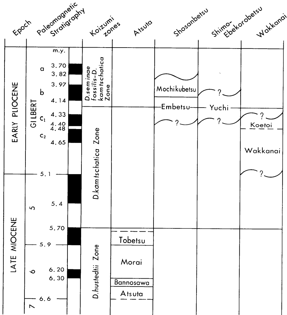
Fig. 24. Correlation chart of the surveyed sequences in the framework of paleomagnetic and diatom stratigraphies.
