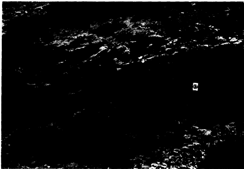
Fig. 11. Thick planar and through cross-stratification in delta plain facies of coarsening-upward cycle at Toyosaki. Shrine gate is 2 m high.
