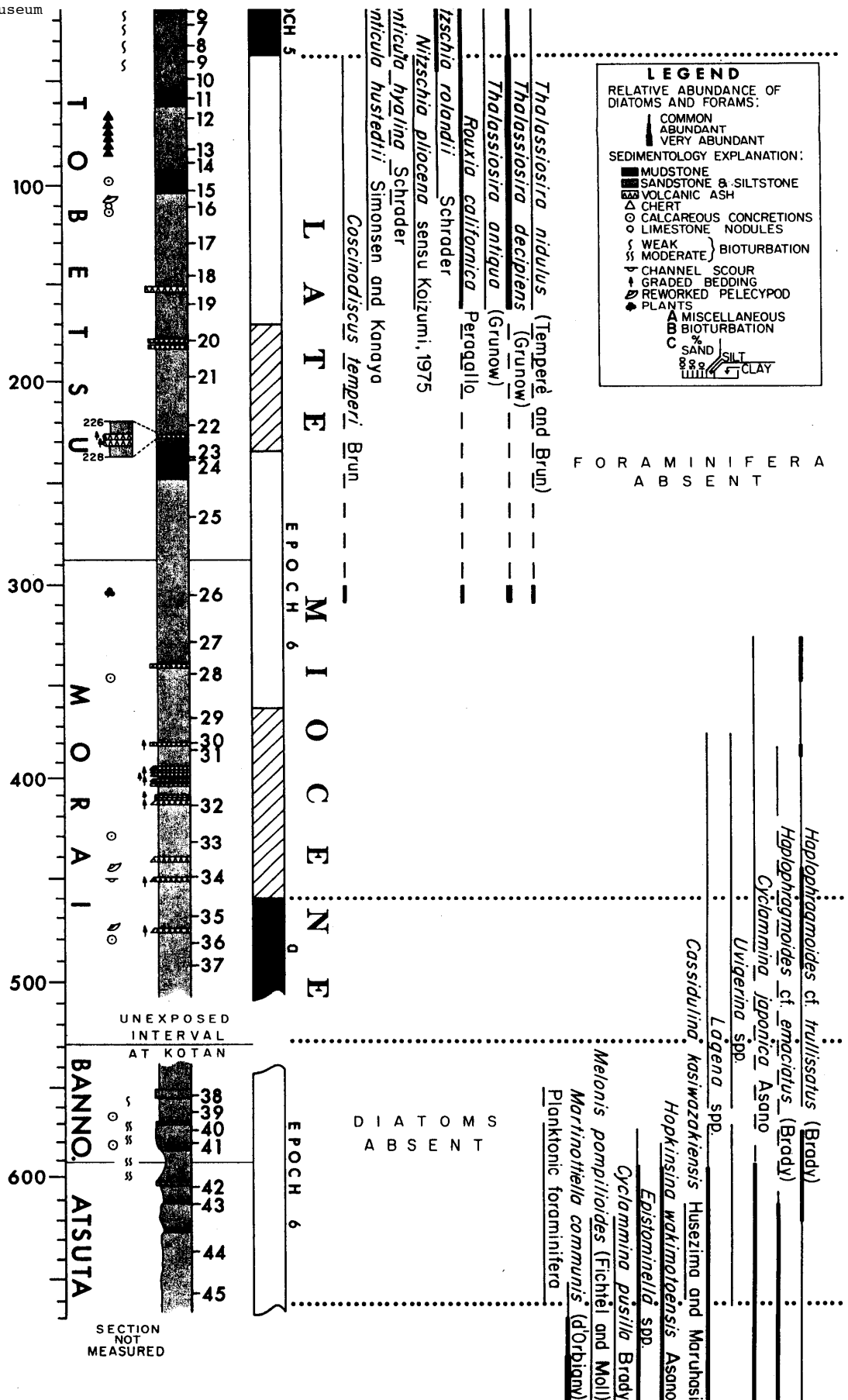
Fig. 22. Composite stratigraphy of the Atsuta section.
