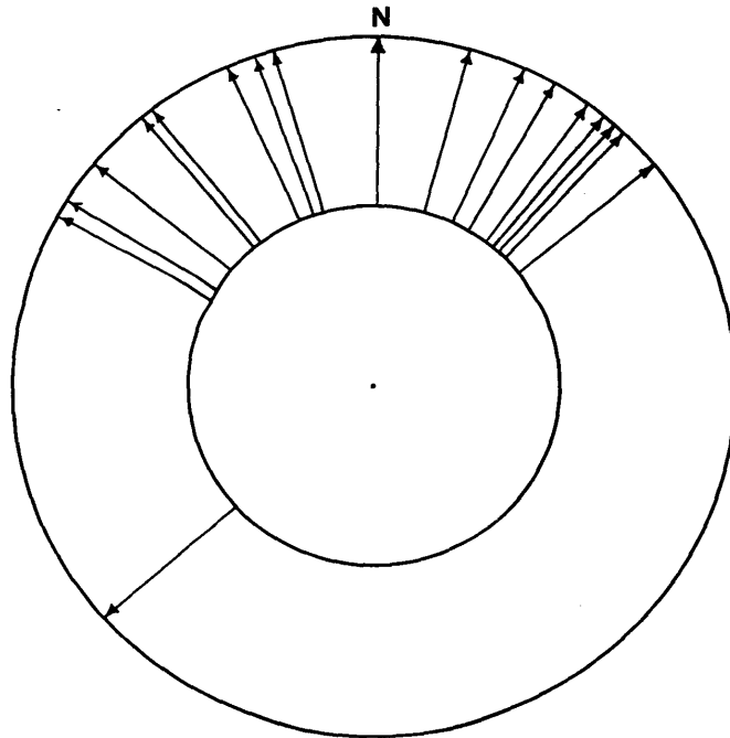
Fig. 12. Paleocurrent diagram of cross-stratification, deltaic sandstones at Toyosaki.
