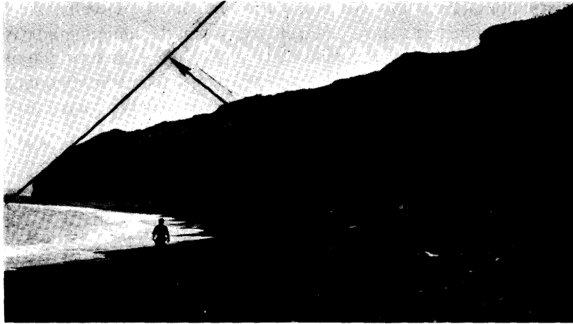
Fig. 10. Coarsening-upward sequence of basal prodelta mudstones, interlayered sandstone-mudstone zone of delta front, and uppermost delta plain sandstone. Arrow shows interval represented by such a sequence. Sandstones below in right foreground represent turbidites. Toyosaki.
