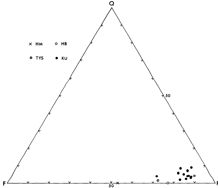
Fig. 13. Ternary diagram showing sandstone compositions. Q: quartz, F: feldspar, R: rock fragments. HM: Morai Formation, HB: Bannosawa Formation, TYS: sandstone member of the Embetsu Formation, KU: Kotanbetsu Formation.
