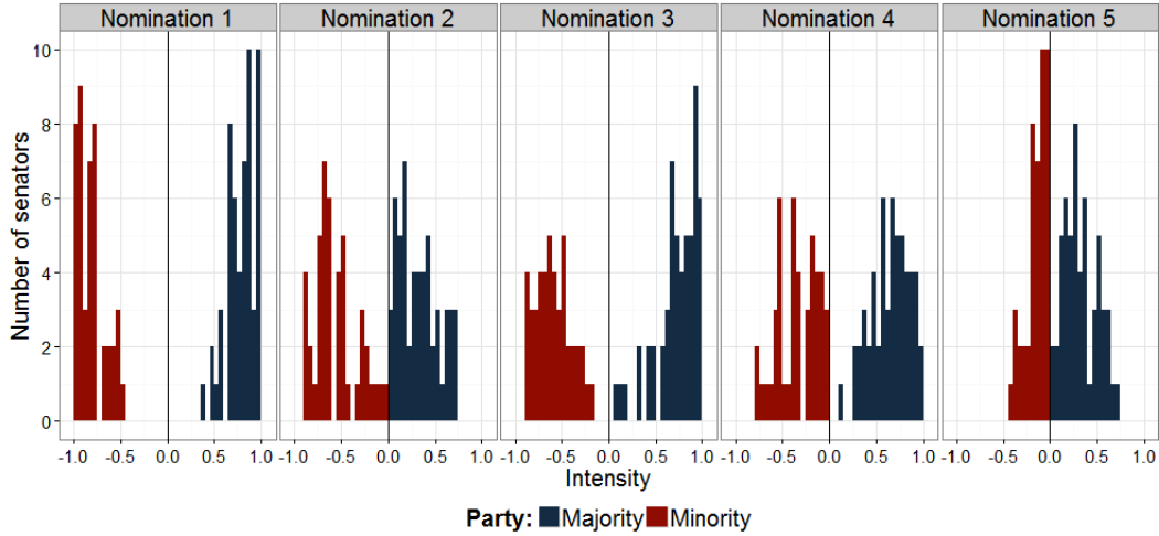
Figure 4: Example of value draws' histogram for \rho = .5 and \rho_{inter} = .3 : number of values within bins of .05.
