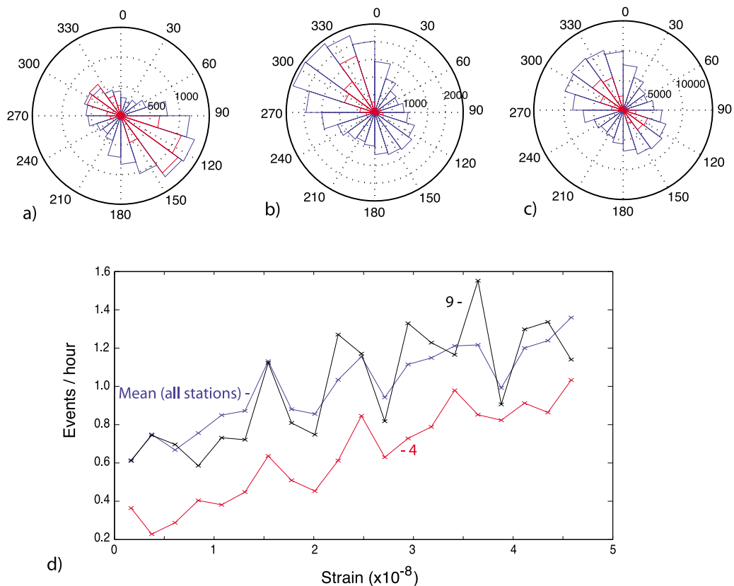
Figure 8. Rose diagrams depicting the phase of each Ishmael-detected tremor (blue) and RMS phase lag for all 4 day periods exhibiting a correlation >0.5 (red). The latter is scaled 60X. (a) Tremor activity at station 4, which peaks during periods of compressional strain, with a mean resultant phase angle of 139^\circ . (b) Tremor recorded at station 9, with a mean resultant phase of 307^\circ . (c) A composite of tremor activity from all stations with tremor occurrence dominantly during periods of both increasing extensional and compressional strain. (d) Tremor occurrence rates for stations 4 (red) and 9 (black) and a mean of all stations (blue). Occurrence rates were binned based on the strain amplitude during the tidal half-cycle in which the event occurred and are normalized based on total time within each amplitude bin. Tremor amplitude and duration (not shown) exhibit a similar positive linear trend with respect to increasing tidal amplitude.
