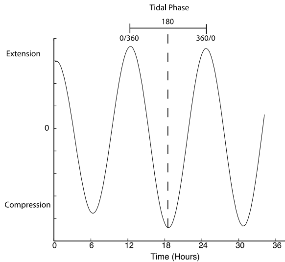
Figure 6. Illustration of a 36 h window of the tidal strain time series. The tidal phase of each individual tremor detection is determined by assigning a phase angle based on the start time of the tremor event. Phase angles are assigned based on 180^\circ as the peak in compressional strain for a given tidal cycle, with 0^\circ or 360^\circ denoting the peak in extensional strain. Phase is assigned independent of strain value.
