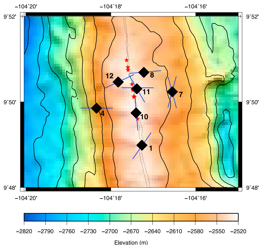
Figure 3. Polarization results for all fourth deployment stations. Station orientations determined from the analysis of regional earthquake signals. Stations 7 and 11 exhibit two dominant polarization azimuths. Red stars represent locations of known high-temperature hydrothermal vent systems, and gray lines denote the AST [Fornari et al. , 1998a].
