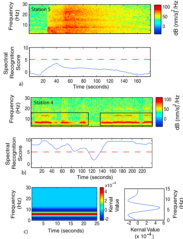
Figure 4. Spectrograms showing (a) a broadband arrival (P, S, and T phases) from a regional earthquake and (b) that of a 4–8 Hz tremor signal. (c) Cross correlation of a 25 s duration, hat-shaped kernel produces a time series of recognition scores. A detection threshold (red line) is then applied to create a series of detections.
