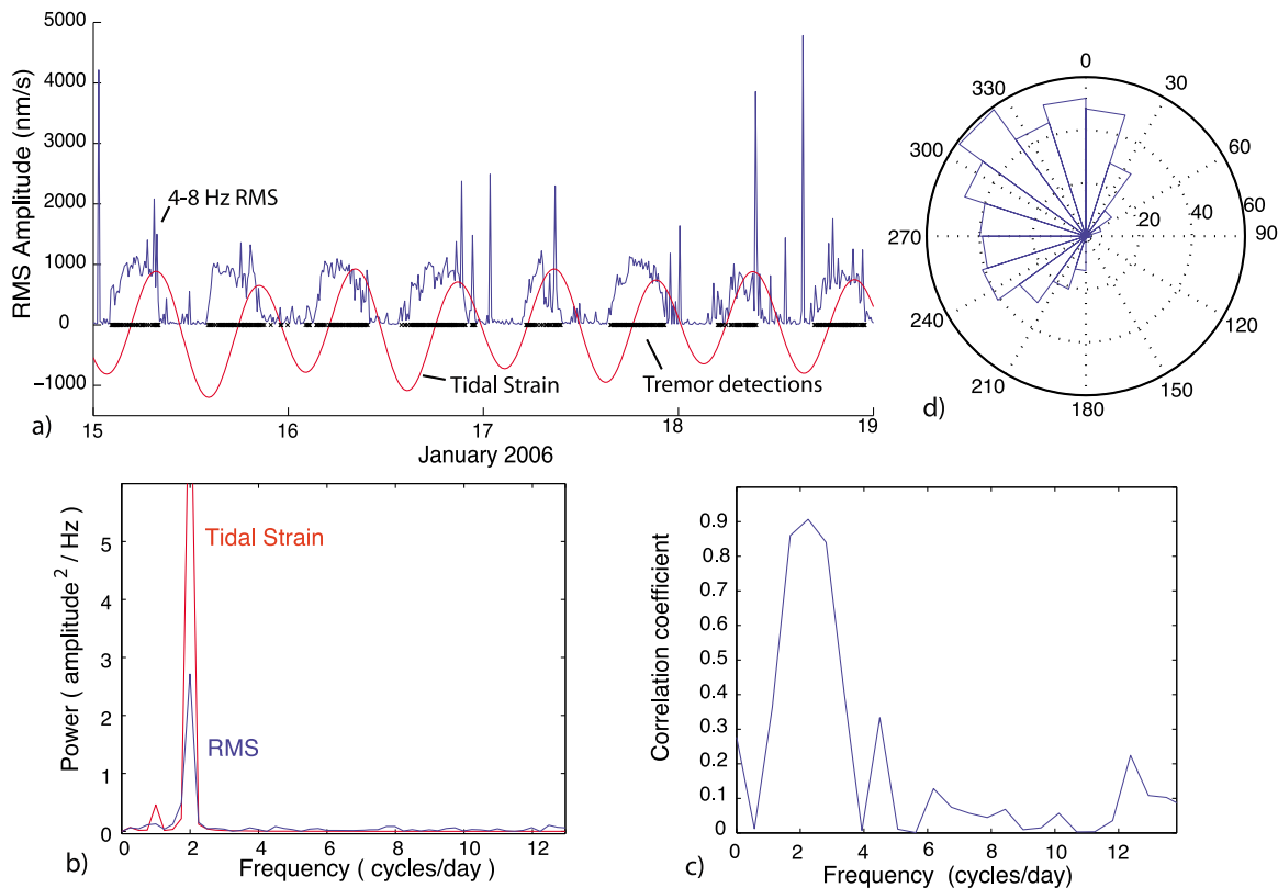
Figure 7. An example of a 4 day interval with a high correlation between RMS amplitudes and tidal strain. All of the data presented were recorded by on-axis station 9 between 15 and 19 January 2006 (deployment 3). (a) RMS velocity amplitude shown in blue. Tidal strain is plotted in red and ranges \pm 2.5 \times 10^{-8} . Tremor detections are plotted as individual crosses. (b) Fast Fourier transform (FFT) of tidal strain (red) and RMS amplitude (blue), both exhibiting peak spectral power at \sim 2 cycles/d. (c) Cross-spectral power analysis shows RMS amplitude and tidal strain exhibit 0.91 correlation at the frequency of 2 cycles/d. (d) Rose diagram depicting the tidal phase associated with each of the 489 tremor events plotted in Figure 7a. The mean phase angle is 307^\circ with a Schuster p value of \ll 0.001 (significant nonrandom temporal occurrence).
