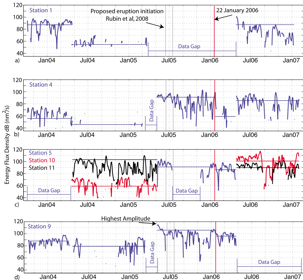
Figure 5. Energy flux density (dB (nm 2 /s)) within Ishmael-detected tremor events integrated over 4 day windows with 50% overlap. Stations (a) 1, (b) 4, (c) 5, and (d) 9. The date of the 22 January 2006 seismic swarm is denoted with a red line. Rubin et al. 's [2008] proposed period of eruption initiation based on 210 Po- 210 Pb data is marked with gray lines. Station 5 recorded the eruption but was not occupied at any other time. As a result, stations 10 and 11 are included in the plot for comparison purposes, as these are the stations in closest proximity to station 5. The highest energy flux is observed at station 9 in May 2005. Horizontal bars represent average energy flux for days with tremor and also indicate the extent of the instrument deployment. Stations recording the eruption are further divided into averages before and after 22 January 2006. Periods without data between deployments as well as gaps in data coverage within deployments are labeled.
