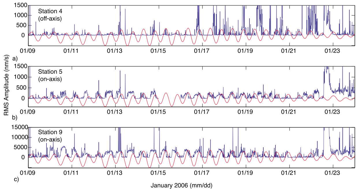
Figure 11. The 10 min RMS amplitudes in the 4–8 Hz band, plotted in blue, for stations (a) 4, (b) 5, and (c) 9 in the 2 weeks preceding the 22 January 2006 microearthquake swarm [Tolstoy et al. , 2006]. Tidal strain is plotted in red and ranges \pm 2.5 \times 10^{-8} . Beginning on 10 January, the phase-shifted correlation between the RMS velocity amplitudes and the tidal time series are greater than 0.90 for station 5 (through 18 January) and station 9 (through 20 January).
