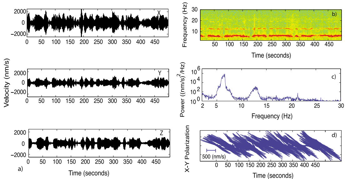
Figure 2. A typical tremor event recorded on OBS stations. Spectra were recorded at station 4 (deployment 3) on 4 May 2005 at 2047:28 UT. (a) X, Y, and Z components of seismic signal. (b) Spectral signature of tremor with fundamental frequency near 6 Hz and harmonic near 12 Hz. Spectrogram parameters are hamming window length of 512 samples with a 256 sample overlap, using 512 frequency points in the Fourier transform at a sampling frequency of 125 Hz. (c) Spectral power ((\text{nm/s})^2/\text{Hz}) for 500 s window shown in spectrogram using Welch's method averaging eight windows with 50% overlap and 4096 points in the zero-padded FFT. (d) The instantaneous polarization on the X-Y plane in time.
