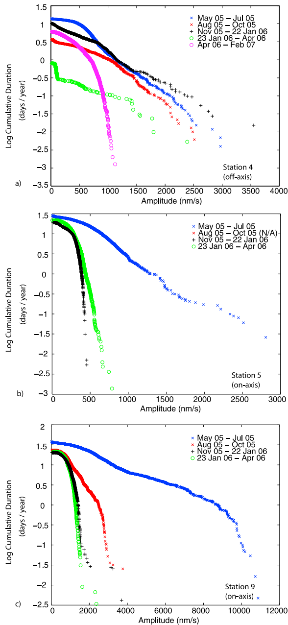
Figure 10. Duration-amplitude distributions of deployment 3 tremor activity recorded at stations (a) 4, (b) 5, and (c) 9. Blue represents activity between May and July 2005. Red represents activity between August 2005 and October 2005, during which time there are no data available for station 5. Black denotes the period between November 2005 and 22 January 2006, with the activity between 23 January and April 2006 shown in green. For station 4, which was reoccupied during the 4th deployment, data from April 2006 to February 2007 are also shown in magenta. Durations have been normalized based on the length of each monitoring period and are in units of cumulative days of tremor per year of observation.
