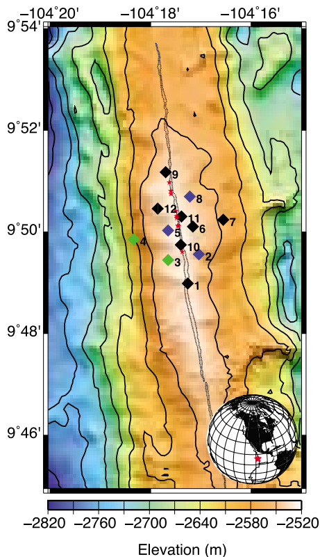
Figure 1. Locations of the 12 unique OBS stations along the ridge crest plotted along with locations of known high-temperature hydrothermal vent systems (red stars). Black diamonds denote stations dominated by tremor occurrence during periods of extensional strain. Green diamonds denote stations dominated by tremor occurrence during periods of compressional strain. Blue diamonds denote stations in which tremor occurrence is temporally nonrandom in both extensional and compressional strain regimes. The periods of active monitoring at each station are in Table 1. Gray lines denote the AST [Fornari et al., 1998a].
