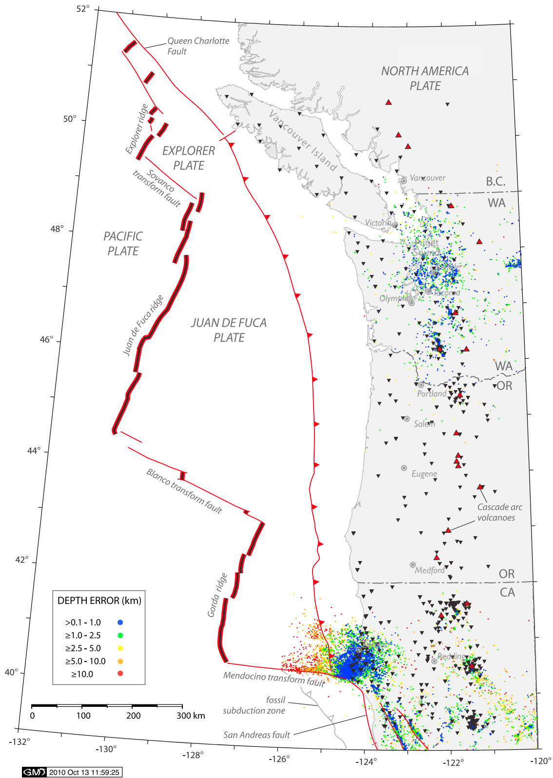
Figure 2. Map showing ANSS Wadati-Benioff epicenters colored by depth error (depth error data not available for CNSN catalog). Current ANSS and CNSN seismicograph stations denoted by inverted black triangles. (See Figure 1 for base map notes.)
