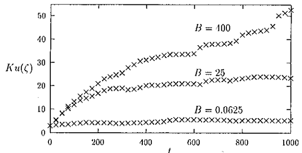
FIG. 7. The kurtosis of vorticity vs time, for the three runs A, D, and F (cf. Table I).
