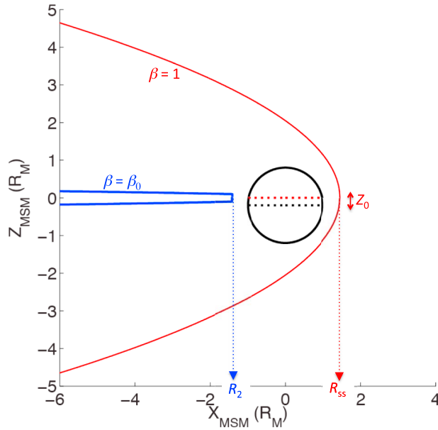
Figure 4. Cross section in the X_{\text{MSM}}-Z_{\text{MSM}} plane of the magnetopause and magnetotail current regions in the paraboloid magnetospheric model. R_{\text{SS}} is the magnetopause subsolar distance, and R_2 is the distance to the inner edge of the tail current sheet. At R_2 the current sheet half thickness is D_D . The magnetopause is the \beta = 1 paraboloid of revolution about the X_{\text{MSM}} axis; the parameter \gamma controls the flaring ( \gamma = 1 ). The tail current sheet is symmetric about the Z_{\text{MSM}} = 0 plane. In an X_{\text{MSM}}-Z_{\text{MSM}} plane the boundary of the current sheet tailward of R_2 is described by the \beta = \beta_0 parabola. The black circle denotes the planetary outline. At Mercury the dipole origin is offset northward by Z_0 from the planetary center as shown in the sketch.
