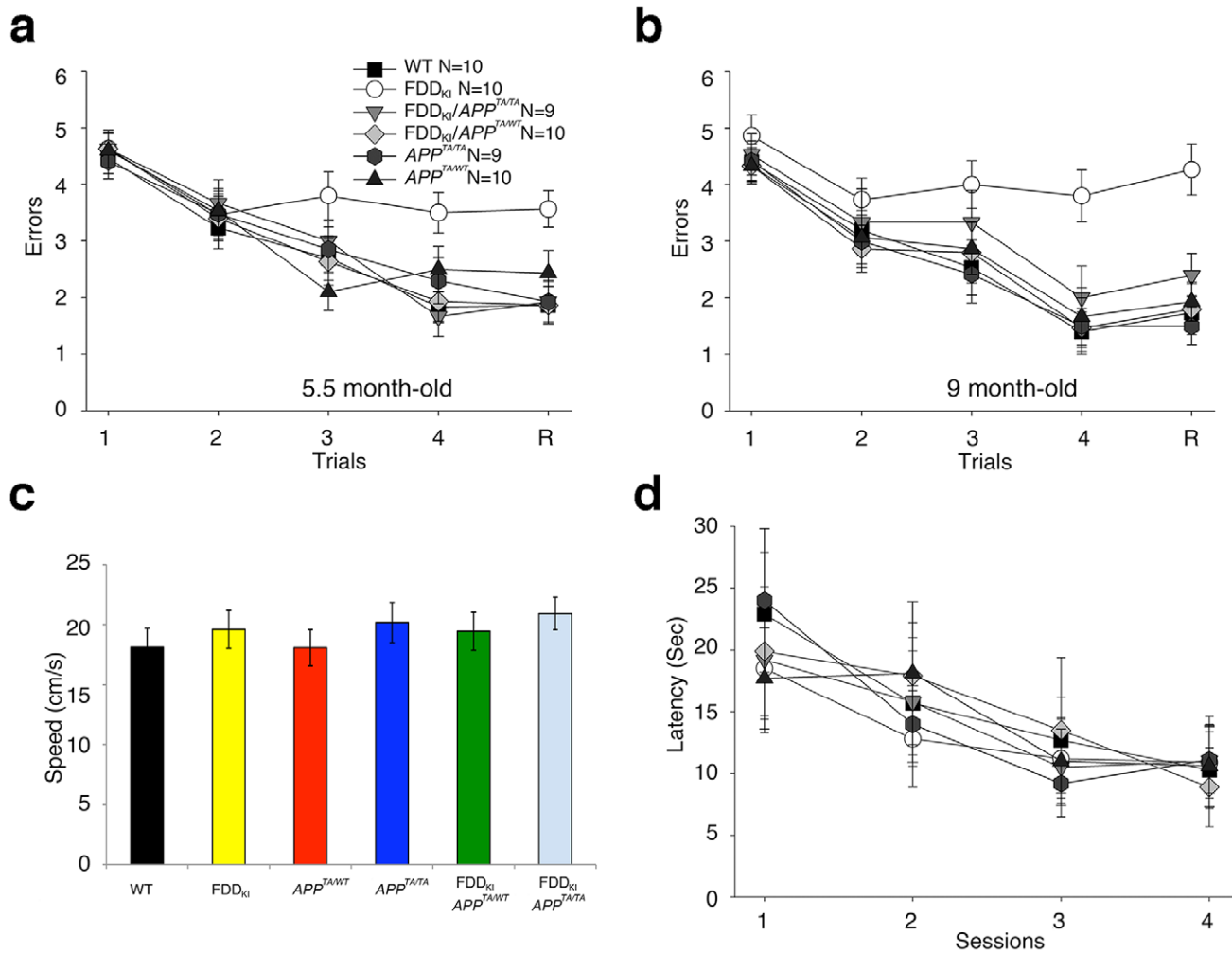
Figure 2. A Thr 668 Ala mutation on APP prevents the short-term memory deficit of FDD K1 mice. (a and b) In RAWM testing, FDD K1 /APP TA/TA , FDD K1 /APP TA/WT , APP TA/TA , APP TA/WT mice made the same number of errors as WT mice at both 5.5 months and 9 months of age. At 5.5 months of age, FDD K1 mice made significantly more errors at A4 (versus FDD K1 /APP TA/TA P=0.0007 ; versus FDD K1 /APP TA/WT P=0.0028 ; versus WT P=0.0005 ) and R (versus FDD K1 /APP TA/TA P=0.0017 ; versus FDD K1 /APP TA/WT P=0.0005 ; versus WT P=0.0005 ) (a). Similar results are found at 9 months of age; FDD K1 mice made significantly more errors at A4 (versus FDD K1 /APP TA/TA P=0.0004 ; versus FDD K1 /APP TA/WT P=0.019 ; versus WT P=0.0003 ) and R (versus FDD K1 /APP TA/TA P=0.0006 ; versus FDD K1 /APP TA/WT P=0.0004 ; versus WT P<0.0001 ). Thus, the APP TA/TA and APP TA/WT point mutations prevent the development of working memory deficits in FDD K1 mice (b). (c and d) WT, FDD K1 , FDD K1 /APP TA/TA , FDD K1 /APP TA/WT , APP TA/TA and APP TA/WT mice have similar speed (c) and need similar time (d) to reach a visible platform. doi:10.1371/journal.pone.0057120.g002
