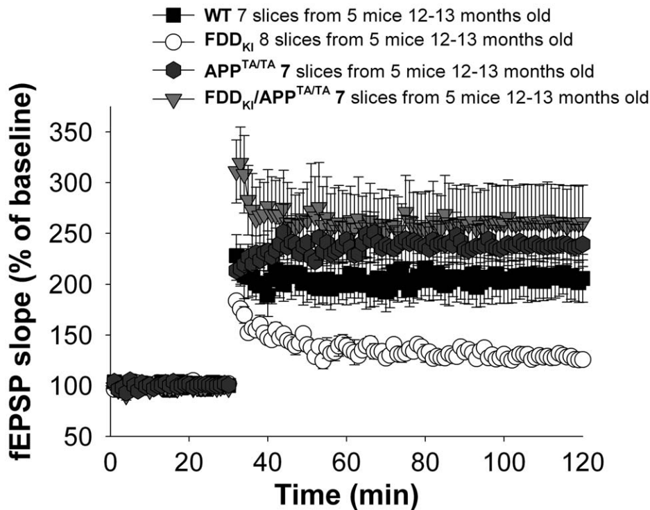
Figure 3. A Thr 668 Ala mutation on APP prevents the synaptic deficits of FDD KI mice. Normal LTP in FDD KI /APP TA/TA and APP TA/TA compared with WT mice by two-way ANOVA (FDD KI /APP TA/TA versus WT mice: F(1,12) = 1.936 ; P = 0.187 ; APP TA/TA versus WT F(1,12) = 0.989 ; P = 0.338 ). Two-way ANOVA shows impaired LTP in FDD KI mice when compared with WT ( F(1,13) = 15.125 ; P = 0.002 ), to FDD KI /APP TA/TA ( F(1,13) = 12.759 ; P = 0.004 ) or to APP TA/TA mice littermates ( F(1,13) = 22.396 ; P < 0.0001 ). doi:10.1371/journal.pone.0057120.g003
