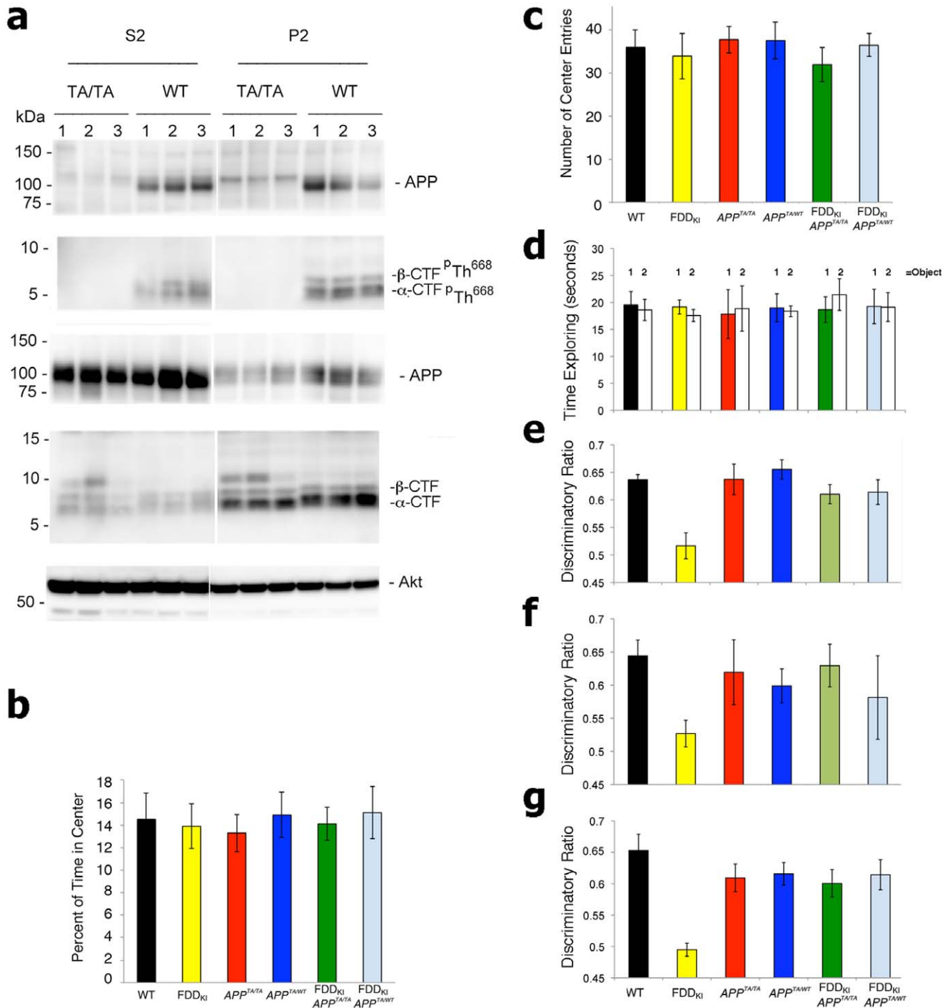
Figure 1. A Thr 668 Ala mutation on APP prevents the object recognition memory deficit of FDD KI mice. (a) Western blot analysis of hippocampal synaptosomal preparations shown that the Thr to Ala mutation abolishes phosphorylation of Thr 668 (APP P Th 668 ). Interestingly, only the mature form of APP (mAPP) and not the immature (imAPP), is found phosphorylated on this Thr in hippocampal synaptic fractions of WT mice. (b and c) Open field is a sensorimotor test for habituation, exploratory, emotional behavior, and anxiety-like behavior, in novel environments. The percent of time in the center (b) and the number of entries into the center (c) are indicators of anxiety levels. The more the mouse enters the center and explores it, the lower the level of anxiety-like behavior. Since the FDD KI , FDD KI /APP TA/TA , FDD KI /APP TA/WT , APP TA/TA , APP TA/WT mice are similar to the WT animals there is no deficit or excess of anxiety. (d) All six genotypes (WT, FDD KI , FDD KI /APP TA/TA , FDD KI /APP TA/WT , APP TA/TA , APP TA/WT ) mice spent similar amounts of time exploring the two identical objects on day 1. (e) FDD KI /APP TA/TA and FDD KI /APP TA/WT mice behaved similarly to WT mice and prevented the deficit in the NOR tests found in FDD KI mice at 6 months of age (FDD KI versus FDD KI /APP TA/TA P=0.011; FDD KI versus FDD KI /APP TA/WT P=0.0083; FDD KI versus WT P<0.001), (f) 9 months of age (FDD KI versus FDD KI /APP TA/TA P=0.01; FDD KI versus FDD KI /APP TA/WT P=0.347; FDD KI versus WT P=0.000995), and (g) 12 months of age (FDD KI versus FDD KI /APP TA/TA P=0.0003; FDD KI versus FDD KI /APP TA/WT P=0.0002; FDD KI versus WT P<0.0001). Thus the APP TA point mutation prevented the novel object recognition deficit of FDD KI mice. doi:10.1371/journal.pone.0057120.g001
