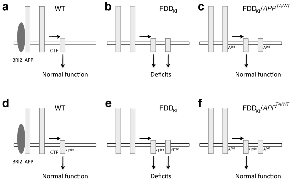
Figure 4. Model depicting the mechanisms by which Thr 668 may lead to memory and synaptic plasticity deficits. (a and b), Due to loss of BRI2 protein, APP processing is increased during synaptic transmission and memory acquisition in FDD leading to increased production of \beta -CTF. This event compromises synaptic plasticity and memory acquisition leading to memory deficits. (c), Thr 668 is essential for the pathogenic role of \beta -CTF, as shown by the evidence that mutating this residue into an Ala prevents development of memory/synaptic deficits. (d–f), Phosphorylation of Thr 668 may be required or facilitate the synaptic-toxic role of \beta -CTF, since the Thr 668 Ala mutation prevents phosphorylation. doi:10.1371/journal.pone.0057120.g004
