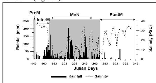
Figure 2 Variation in Salinity and Rainfall in Mandovi estuary. Where 143-147 (PreM), 148-174 (InterM), 175-272 (MoN) and 273-334 (PostM).
