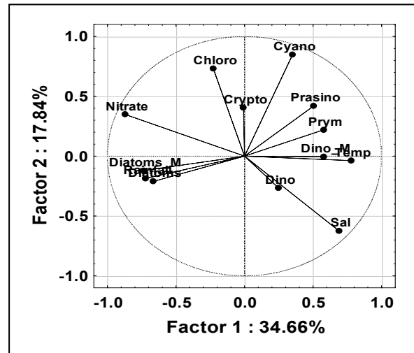
Figure 8A Principal Component Analysis ordination diagram relative to data on absolute contribution of phytoplankton groups by CHEMTAX and microscopy and physicochemical parameter during Intermonsoon in the Mandovi estuary. Symbols represents Dino-dinoflagellates; Cyano-cyanobacteria; Crypto-cryptophytes; Chloro-chlorophytes;Prym-prymnesiophytes; Prasino-prasinophytes; Diatom_M-diatoms by microscopy; Dino_M-dinoflagellates by microscopy; Temp-temperature and Sal-salinity.
