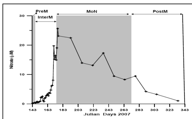
Figure 3 Variation in Nitrate in Mandovi estuary. Where 143-147 (PreM), 148-174 (InterM), 175-272 (MoN) and 273-334 (PostM).
