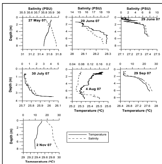
Figure 4 Temperature and salinity variations in the Mandovi estuary.
