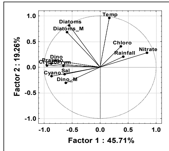
Figure 8B Principal Component Analysis ordination diagram relative to data on absolute contribution of phytoplankton groups by CHEMTAX and microscopy and physicochemical parameter during Monsoon in Mandovi estuary. Symbols are represented with the same used in Figure 8A.
