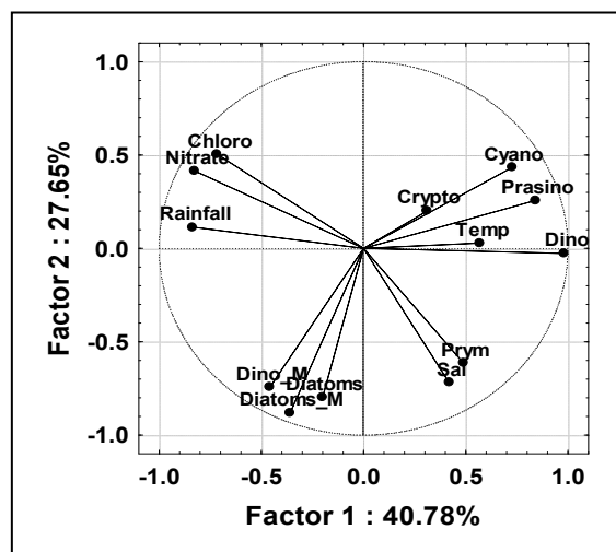
Figure 8C Figure 8C Principal Component Analysis ordination diagram relative to data on absolute contribution of phytoplankton groups by CHEMTAX and microscopy and physicochemical parameter during Post-monsoon in the Mandovi estuary. Symbols are represented with the same used in Figure 8A.
