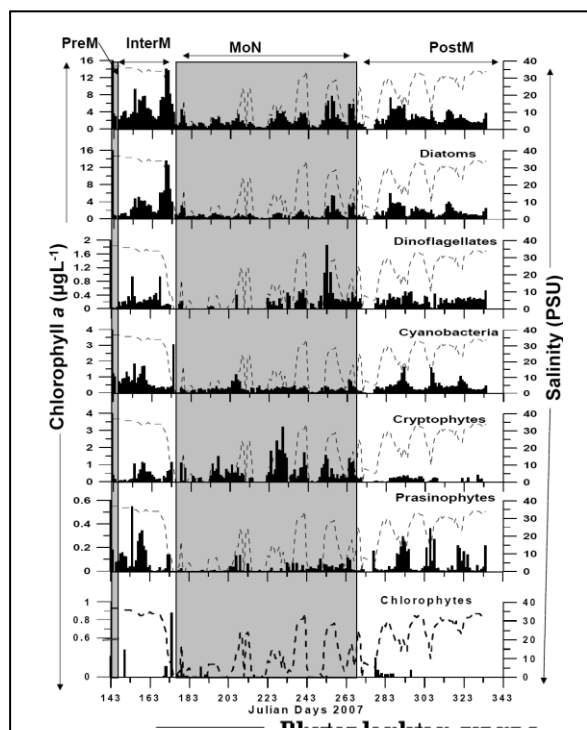
Figure 6 Phytoplankton groups revealed by CHEMTAX and Salinity variation.
