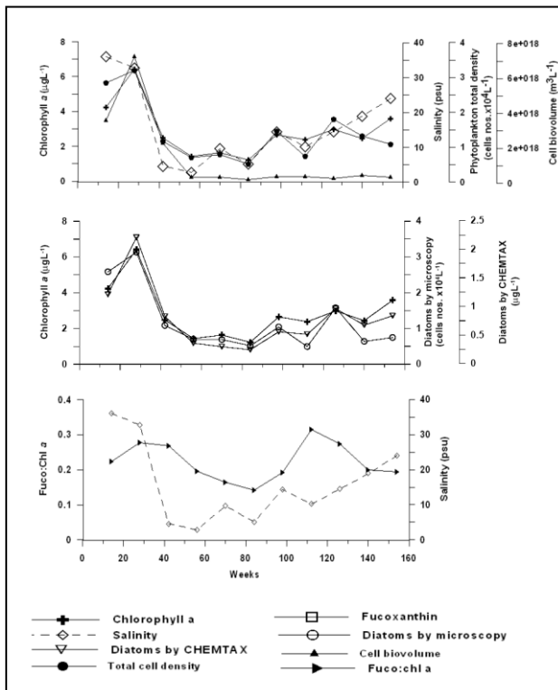
Figure 7 Pigment : chl a ratio and salinity in Mandovi estuary during the Monsoon season.
