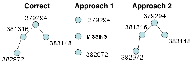
Figure 6. An example to explain the superiority of Approach 2 against Approach 1 when missing messages exist
