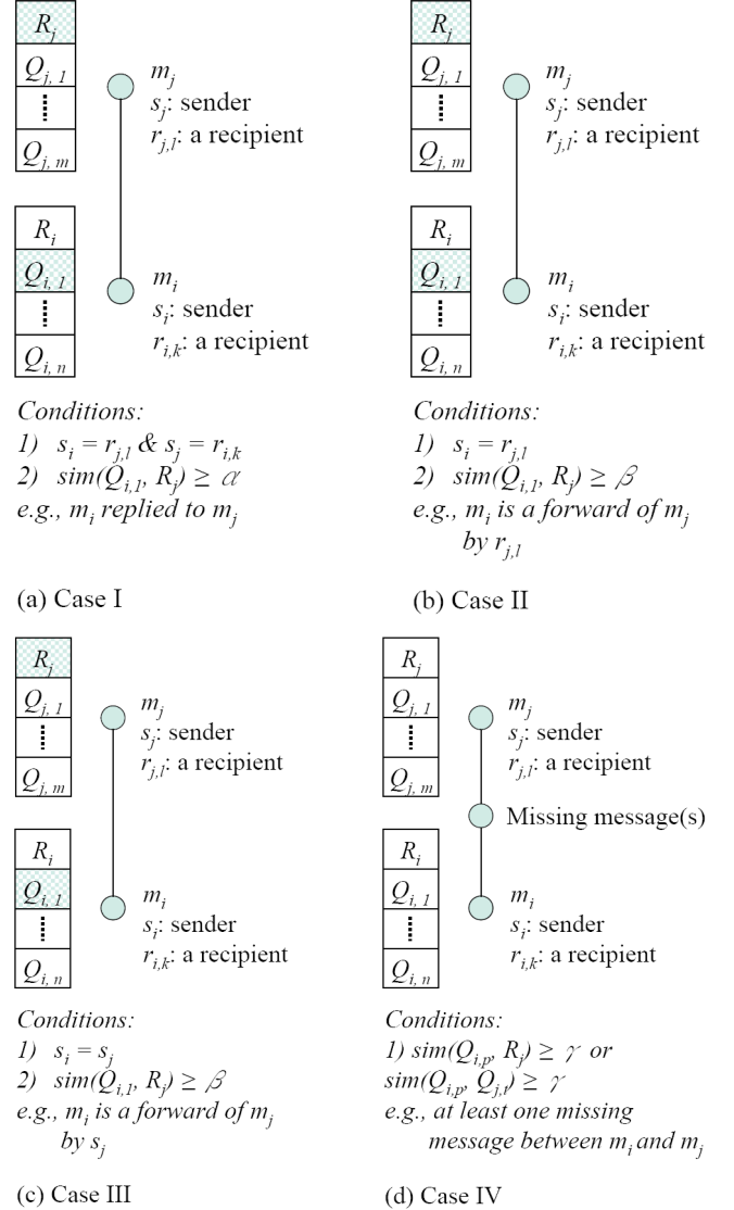
Figure 1. Illustrations of Case I-IV in FindParent ( m_i, T )
