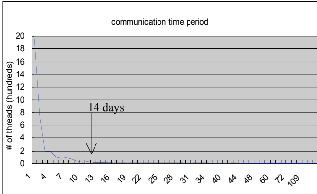
Figure 3. The distribution of communication time period of threads generated by Approach 1
