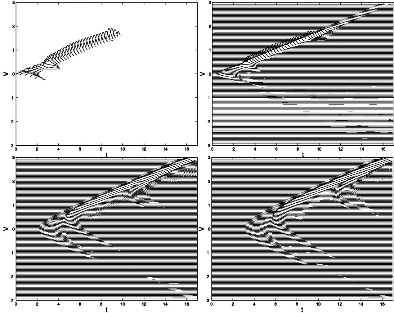
Figure 4. Array of velocity records for different distances from fault. This is a large event in the model, with a nearly unilaterial rupture. Note the large-scale change relative to the previous small event in Figure 3. The vertical axis is velocity, while the horizontal axis is time. Neighboring records are offset in the vertical direction by a constant velocity increment, to more easily see the correlations. From left to right, from top to bottom, the distances of the arrays from the fault are \Delta_y = 0, 0.25, 2, 3 , respectively. Thus the top left panel shows the motions on the fault, and the other panels show the radiated waves at increasing distances from the fault. For the fault motions in the top left panel, we see a unilaterial rupture with varying slip and varying rupture velocity. The varying slip can be seen by the varying areas under the curves, which are the slip. The varying rupture velocity can be seen by the varying slopes between when neighboring parts of the fault initiate slip.
