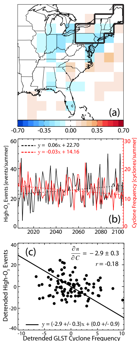
Fig. 8. Long-term trends and correlations between summer (JJA) 2006–2100 GLST cyclone frequency and high-O 3 events in the RCP 4.5* (X3*) warming scenario in which ozone precursor emissions are held constant at 2005 levels. High-O 3 events are defined here as days where the 95th percentile in the 1986–2005 period is exceeded (see Sect. 4 for details). (a) Correlation of the yearly values between the number of high-O 3 events and the number of storms tracking through the GLST in summer (JJA); solid black line outlines the grid cells in the Northeastern US. (b) The number of summer (JJA) high-O 3 events in the Northeastern US (black) and GLST cyclone frequency (red) as solid lines with significant trends ( p < 0.01 ) from a least-squares regression shown as dashed lines. Equations for significant trends are shown where x as the year subtracted by 2006 (the intercept given is for the year 2006). (c) Scatterplot of high-O 3 events ( n ) and GLST cyclone frequency ( C ) after removing significant trends shown in panel (b). Solid black line is the reduced major axis regression of the detrended data indicating a sensitivity of \partial n/\partial C = -2.9 \pm 0.3 with a correlation ( r ) of -0.18 .
