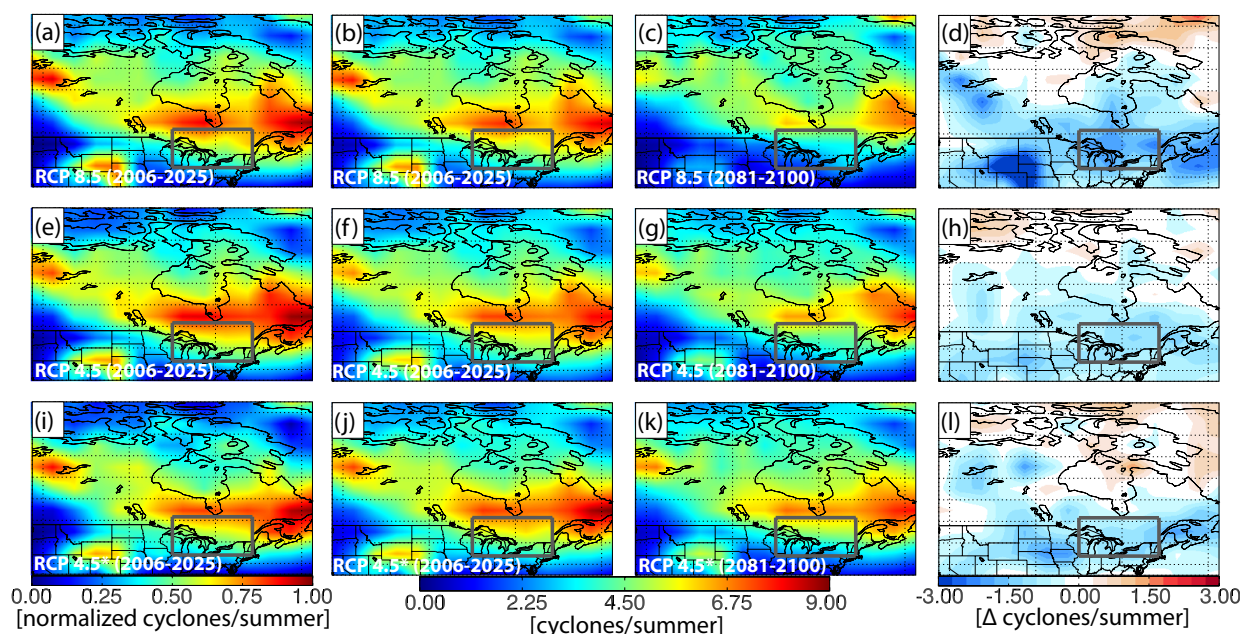
Fig. 6. Spatial distribution of GFDL CM3 cyclone tracks during JJA. Left column (a, e, i) shows the normalized base period (2006–2025), middle left column (b, f, j) shows the base period (2006–2025), middle right column (c, g, k) shows the future period (2081–2100), and the right column (d, h, l) is the difference (Future – Base). First row (a, b, c, d) is the RCP 8.5 scenario, second row (e, f, g, h) is RCP 4.5 ensemble mean, and the third row (i, j, k, l) is RCP 4.5* (Table 1).
