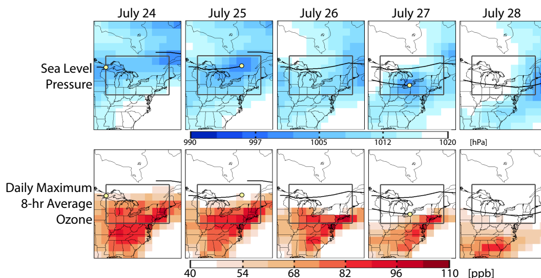
Fig. 1. A clearing event simulated in the GFDL CM3 GCM from 24 July to 28 July for a year selected from the GCM RCP 8.5 simulation. The top row shows the sea level pressure at 9Z and the bottom row shows the daily maximum 8-h average ozone concentration in surface air. The gray box in all panels indicates the GLST and the black lines are storm track. The yellow dot indicates the position of the storm at the current time step. Storm tracks without a yellow dot are storms that still meet the criteria described in Sect. 2.2 but have moved out of the domain.
