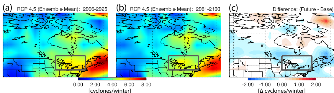
Fig. 5. Spatial distribution of GFDL CM3 cyclone frequencies during winter (DJF) for the RCP 4.5 ensemble mean. (a) Base period: 2006–2025. (b) Future period: 2081–2100. (c) Difference between (a) and (b). Gray box bounds the GLST.
